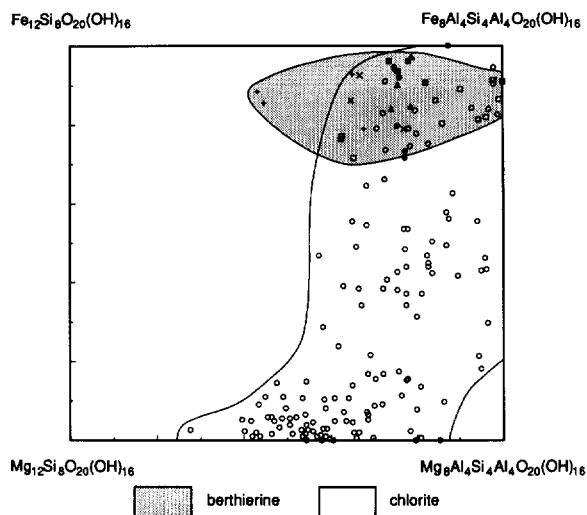
Figure 11. Compositional fields of berthierine and chlorite in a \text{Fe}_{12}\text{Si}_8\text{O}_{20}(\text{OH})_{16} - \text{Mg}_{12}\text{Si}_8\text{O}_{20}(\text{OH})_{16} - \text{Fe}_8\text{Al}_4\text{Si}_4\text{Al}_4\text{O}_{20}(\text{OH})_{16} - \text{Mg}_8\text{Al}_4\text{Si}_4\text{Al}_4\text{O}_{20}(\text{OH})_{16} quaternary diagram. \circ = chlorite from Foster (1962), \square = berthierine from Bhattacharyya (1983), + = berthierine from Hughes (1989), \times = chlorite from Hughes (1989), \bullet = chlorite from this study, \blacksquare = berthierine from this study, \blacktriangle = mixed-layer chlorite/berthierine from this study. All data are normalized on the basis of 20 total tetrahedral and octahedral cations. Minor Mn contents are included with Mg contents, and minor alkali and Ca contents are excluded in the normalization.
