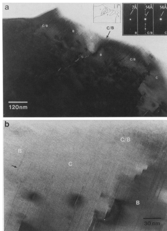
Figure 7. (a) Transmission electron micrograph of a composite chlorite-berthierine grain in sample KC-813. The layers of berthierine (B), chlorite (C), and mixed-layer chlorite/berthierine (C/B) are parallel, but phase boundaries are subparallel to the layers. Insets show electron diffraction patterns characteristic of berthierine, mixed-layer chlorite/berthierine, and chlorite, and a schematic diagram (numbers 1 = C/B, 2 = B, and 3 = C) of the imaged area. (b) Lattice-fringe image of the central part (marked by a black arrow) of (a) showing detailed textures across a high-strain zone consisting of several kink bands and lens-shaped pores that separates packets of berthierine and mixed-layer chlorite/berthierine. Islands and thin packets of 14-Å layers are present within the berthierine crystals.
