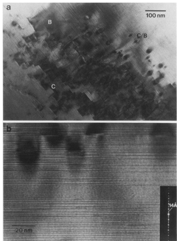
Figure 6. (a) Transmission electron micrograph of a composite chlorite-berthierine grain in sample KC-813 showing a high-strain zone that separates chlorite (C) from berthierine (B) and mixed-layer chlorite/berthierine (C/B). Chlorite layers are highly distorted in the high-strain zone. (b) Lattice-fringe image of the mixed-layer region in (a). Note interstratification of packets of chlorite (wide fringes) and berthierine (narrow fringes) of various thicknesses. Conversions of one layer of chlorite to two layers of berthierine in adjacent layers are common. Areas of high strain contrast are present locally, e.g., upper half of (b), probably due to lateral misfit between chlorite and berthierine layers. Inset shows an electron diffraction pattern of the mixed-layer region.
