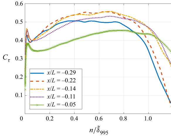
Figure 13. Correlation coefficient C_\tau in the FPG region of the Gaussian bump.
