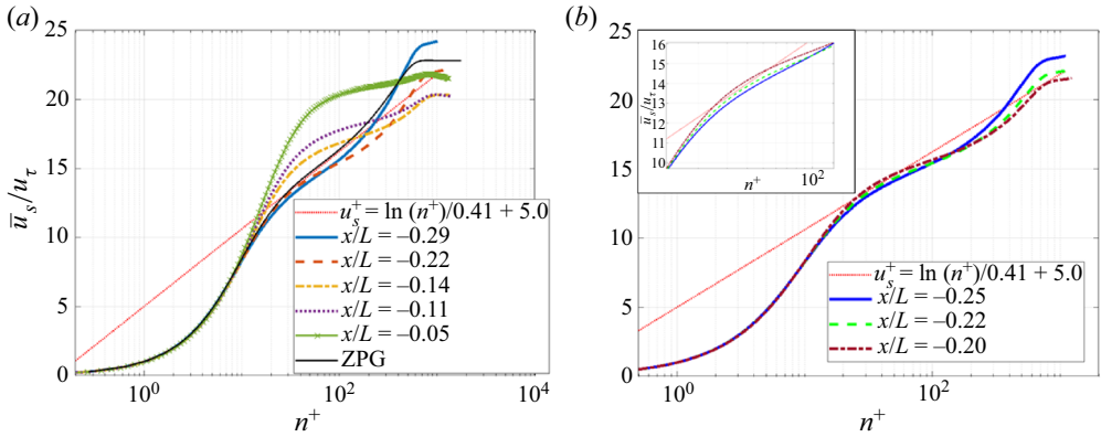
Figure 10. Mean streamwise velocity profiles in the FPG region normalized by wall units. The ZPG profiles are taken from the DNS of Jimenez et al. (2010) at Re_\theta = 1551 .
