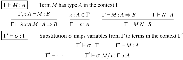
Fig. 1. Typing for STLC, and well-typed substitutions.
