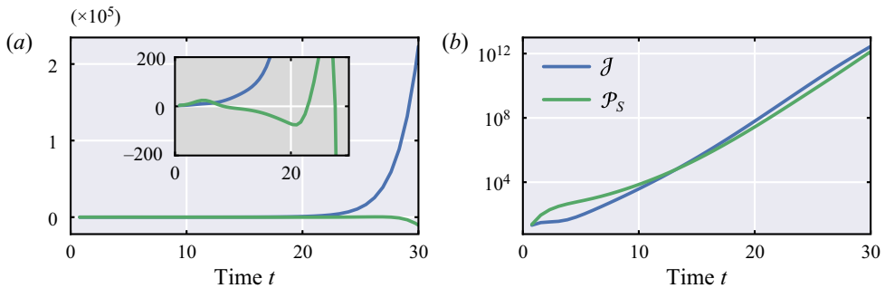
Figure 6. Components of the energy budget for the T = 30 optimal perturbations. Blue: buoyancy flux. Green: shear production. ( a ) Two-dimensional optimal. ( b ) Three-dimensional optimal.
