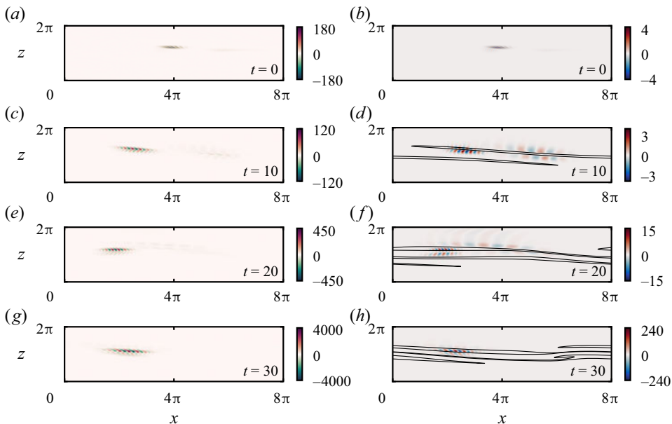
Figure 4. The x - z plane slices of the perturbation spanwise vorticity field \partial u' / \partial z - \partial w' / \partial x (a,c,e,g) and buoyancy b' (b,d,f,h) for the 2-D optimal perturbation (calculated using L_y = 0.1 ) with T = 30 . Alternating spanwise vortices are tilted and distorted by the background shear, as is typical of the Orr mechanism. The black contour on the right surrounds regions of negative (and hence statically unstable) background buoyancy gradient.
