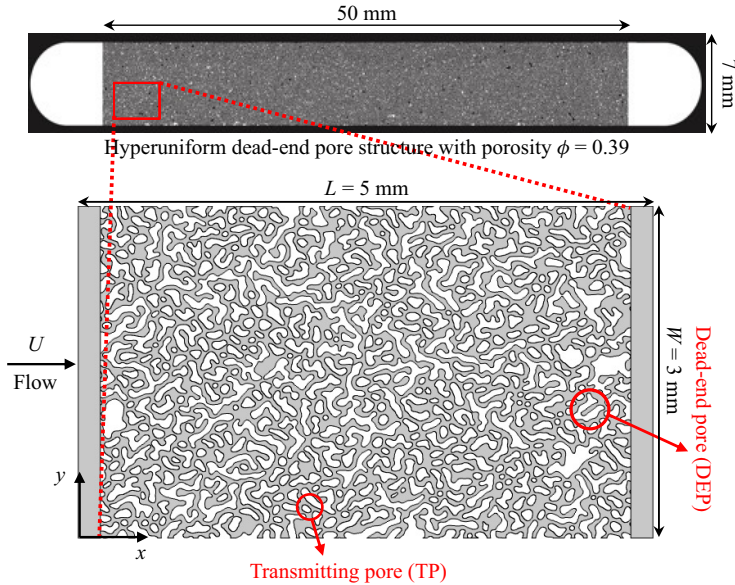
Figure 1. Hyper-uniform porous structure characterised by DEPs and TPs. Computational domain with white spaces indicating solid grains (bottom).
