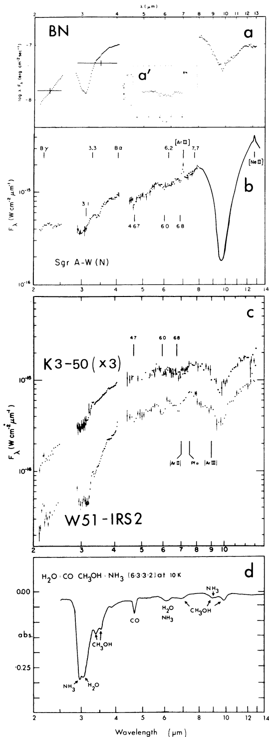
Figure 3. A 2–14 μm spectra of a, a') The BN object reprinted courtesy of Gillet, Jones, Merrill and Stein, 1975 and Russell, Soifer and Puetter, 1977; b) The Galactic Center reprinted from Willner, Russell, Puetter, Soifer and Harvey, 1979; c) K3-50 and W51-IRS2 reprinted from Puetter, Russell, Soifer and Willner, 1979 and; d) The grain mantle analog.
