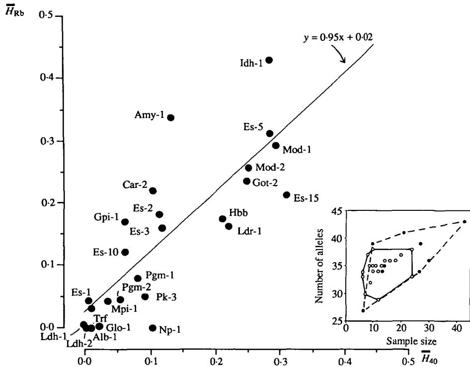
Fig. 3. Correlation of heterozygosity values for polymorphic loci between all-acrocentric ( H_{40} ) and Rb populations ( \bar{H}_{Rb} ). Coefficient of correlation, r = 0.817 ( r = 0, P < 0.001 ). The insert shows the distribution of the number of alleles per sample size for the 25 polymorphic
