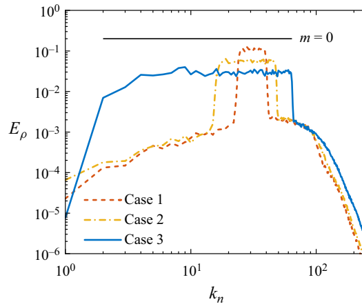
Figure 2. Initial density spectrum at the mixing layer centre.
