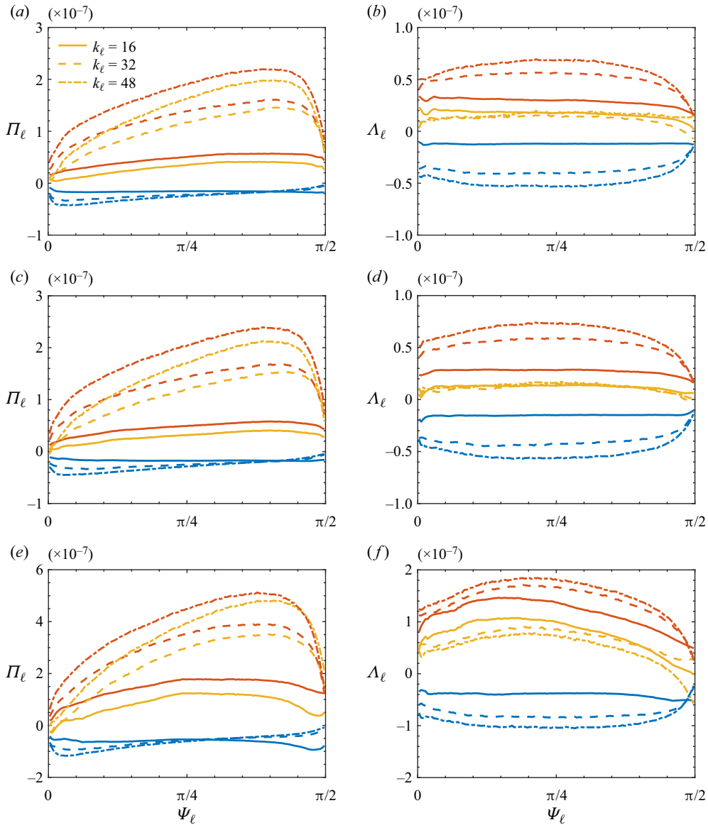
Figure 21. The conditional averaging of (a,c,e) the deformation work, \langle \Pi_\ell \parallel \Psi_\ell \rangle , and (b,d,f) the baropycnal work, \langle \Lambda_\ell \parallel \Psi_\ell \rangle , vs the filtered strain-enustrophy angle, \Psi_\ell . Data are from (a,b) case 1 at \tau = 43.94 , (c,d) case 2 at \tau = 43.67 and (e,f) case 3 at \tau = 44.20 . The yellow, red and blue lines represent the SFS energy fluxed itself, its positive and negative components, respectively. All results in the figure have undergone the same non-dimensionalisation as in figure 13.
