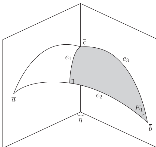
Figure 1. The proof of Lemma 2.3
