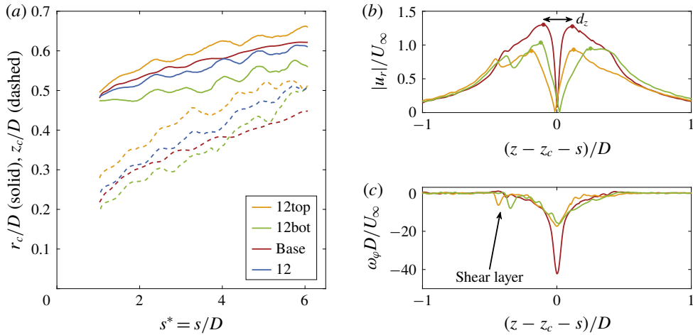
FIGURE 14. Results for Re = 350\,000 . (a) Vortex centre position based on the maximum of the Q -criterion. The blue line depicts the average of 12top and 12bot. (b) Magnitude of radial velocity along a horizontal cut through the vortex centre estimated by the Q -criterion, for s^* = 5 . The distance between the two maxima is defined as the vortex core diameter d_z . (c) Vorticity along a horizontal cut through the vortex core, for s^* = 5 .
