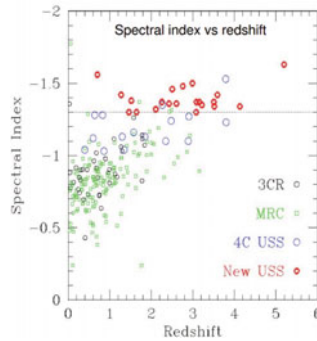
Figure 1. Spectral index vs. redshift for four different samples. Plot from De Breuck et al. (2000).
