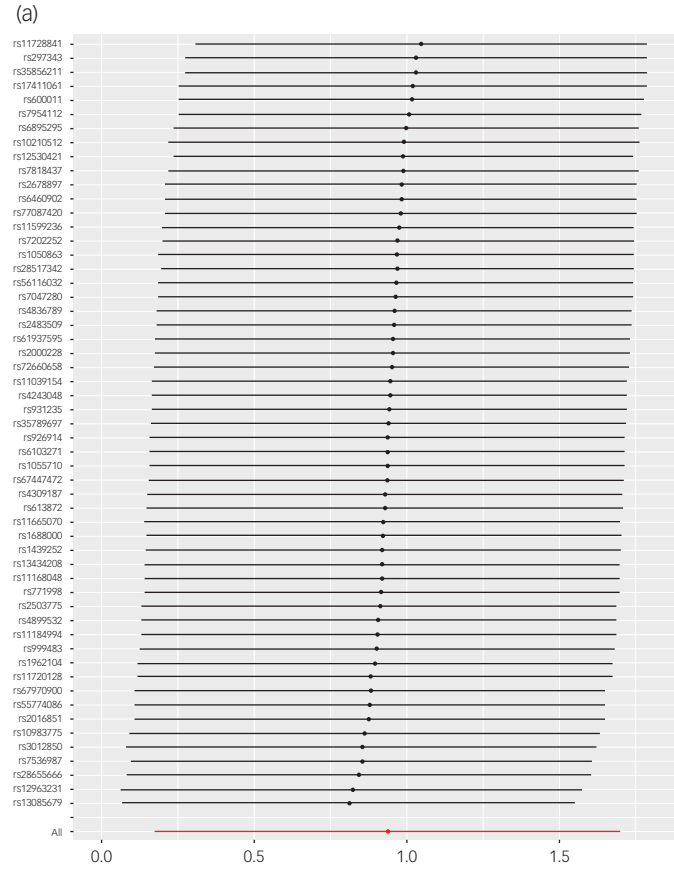
Fig. 3 (a) Leave-one-out sensitivity analysis of the causal effect of mood swings on endometriosis. (b) Leave-one-out sensitivity analysis of the causal effect of major depression on endometriosis.
