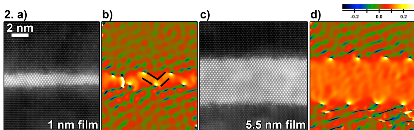
Figure 2. LAADF-STEM images of a) 1 nm c) and 5.5 nm films. b) GPA of of the 1 nm film (strain scale shown above d)) shows formation of a zigzagging strain field (partially outlined with black lines) which arises due to overlap in the film interior of strain fields that originate from dislocations on opposite interfaces. In contrast, transverse dislocation interaction is absent from thicker films, such as the 5.5 nm film in d). Complex strain field formation such as in b) is expected to impact properties in the thinner films. All images are at equal magnification. Image levels are adjusted to enhance contrast.
