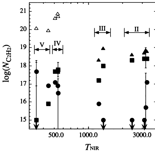
Figure 2. The column densities of \text{C}_2\text{H}_2 molecules in hot ( squares ) and cool ( circles ) layers are plotted against the near-infrared temperature. The hot-layer column densities after correction for dust emission effect are also plotted ( triangle ). The correction may be proper only for the low mass-loss rate stars ( filled triangles ). The error bars given in some data indicate the approximate uncertainty of the results in general. Symbols with arrows are upperlimits.
