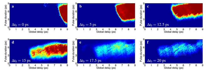
Figure 16. Evolution of the EM radiation pulse emitted by the target. By focusing the main laser onto a wedged target, the probe laser is sent onto the ZnTe crystal with different delays. The horizontal axis represents the relative probe arrival time ( t ) associated with each pixel [31] . \Delta t_0 is the delay between the main and probe laser pulses. From Ref. [31].
