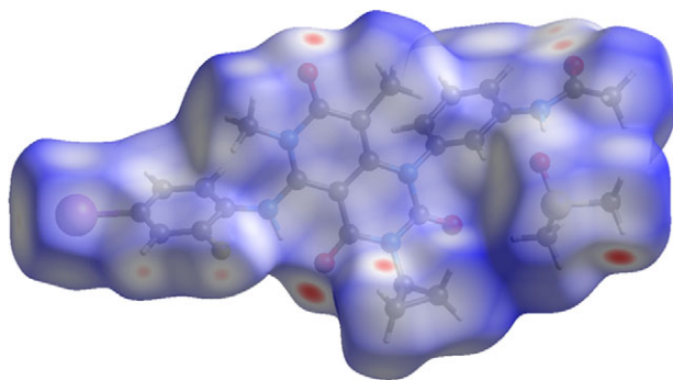
Figure 6. The Hirshfeld surface of trametinib dimethyl sulfoxide. Intermolecular contacts longer than the sums of the van der Waals radii are colored blue, and contacts shorter than the sums of the radii are colored red. Contacts equal to the sums of radii are white. Image generated using CrystalExplorer (Spackman et al., 2021).
