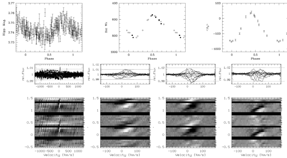
Figure 1. Upper row, from left to right: Hipparcos photometry, equivalent width variability of the combined He I 4009 & 4026 lines (ESPADoNS, open symbols; FEROS, filled symbols), and magnetic data. Lower row, left to right: Exemplary types of line profile variation seen in HR 2949: Balmer wings, Balmer cores (both H \beta ), helium (He I 4388), metal (Fe I 4949).
