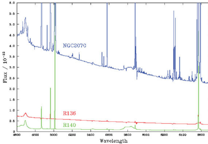
Figure 3. Integrated VLT/MUSE spectrum of NGC 2070 from N. Castro et al. (in prep), highlighting strong blue (He II \lambda 4686 , C III \lambda\lambda 4647-51 ) and yellow (C IV \lambda\lambda 5801-12 ) Wolf-Rayet features, including the individual contributions from R136 and R140.
