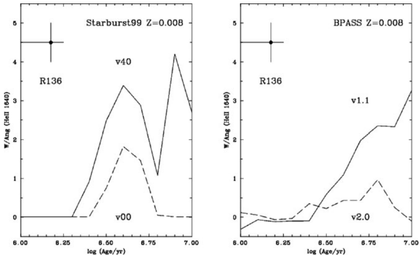
Figure 2. Comparison between observed He II \lambda 1640 emission in R136 (Crowther et al. 2016) and Z = 0.008 instantaneous burst models from (left): Starburst99 (Leitherer et al. 2014) for non-rotating (v00, dashed) and rotating (v40, solid) Geneva single star models with M_{\text{max}} = 120M_{\odot} , (right): BPASS (Eldridge & Stanway 2012, Stanway et al. 2016) close binary models for M_{\text{max}} = 100M_{\odot} (v1.1, solid) and M_{\text{max}} = 300M_{\odot} (v2.0, dashed).
