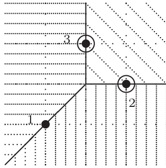
FIGURE 2. The colored fan \bar{\Sigma} of \bar{X} .
