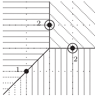
FIGURE 1. The colored fan \bar{\Sigma} of \bar{Q} .
