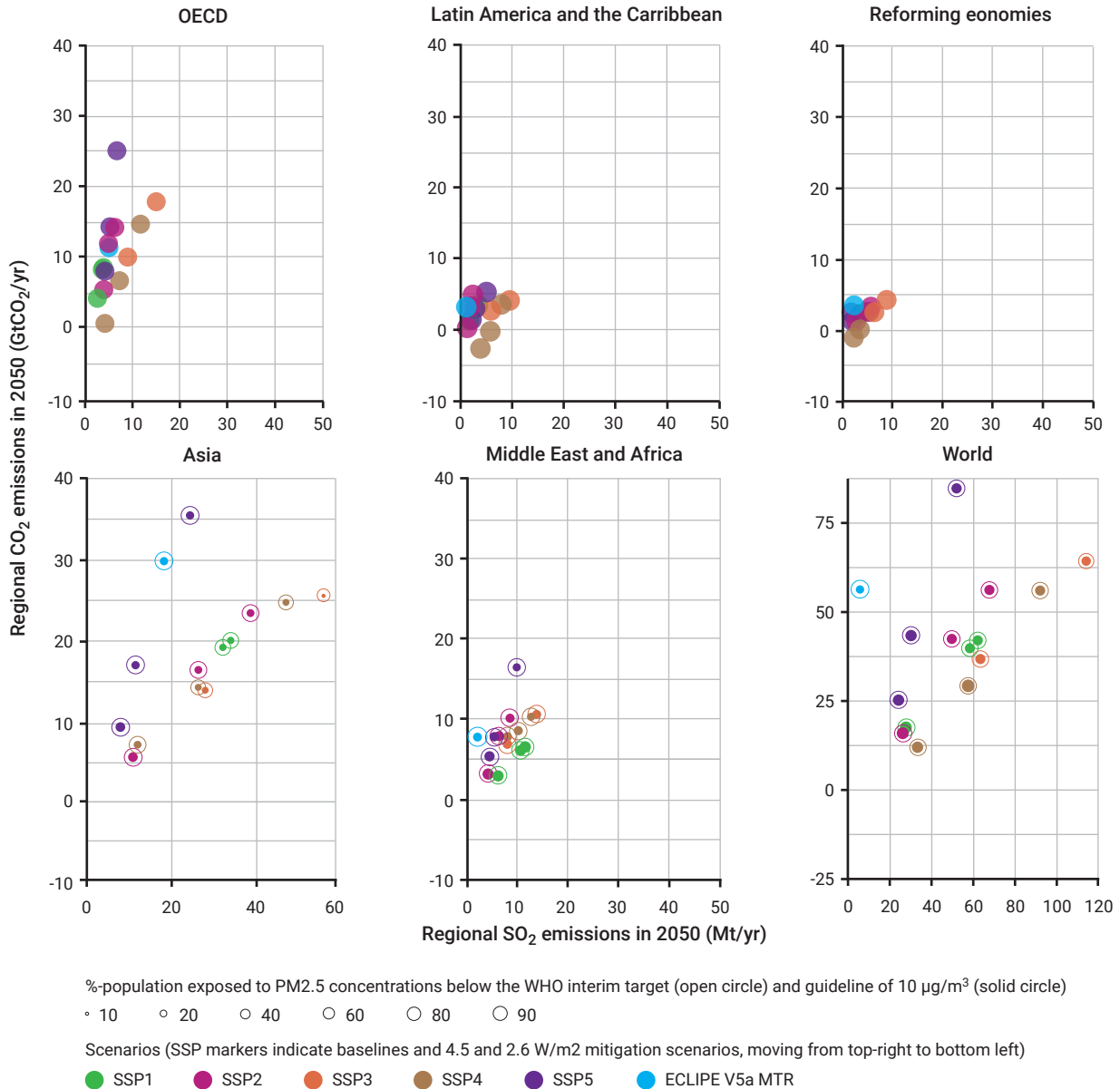
Figure 22.8: Percentage of the population exposed to particulate matter of less than 2.5 \mu\text{m} in diameter ( \text{PM}_{2.5} ) concentrations under the WHO guideline and interim target for 2050
