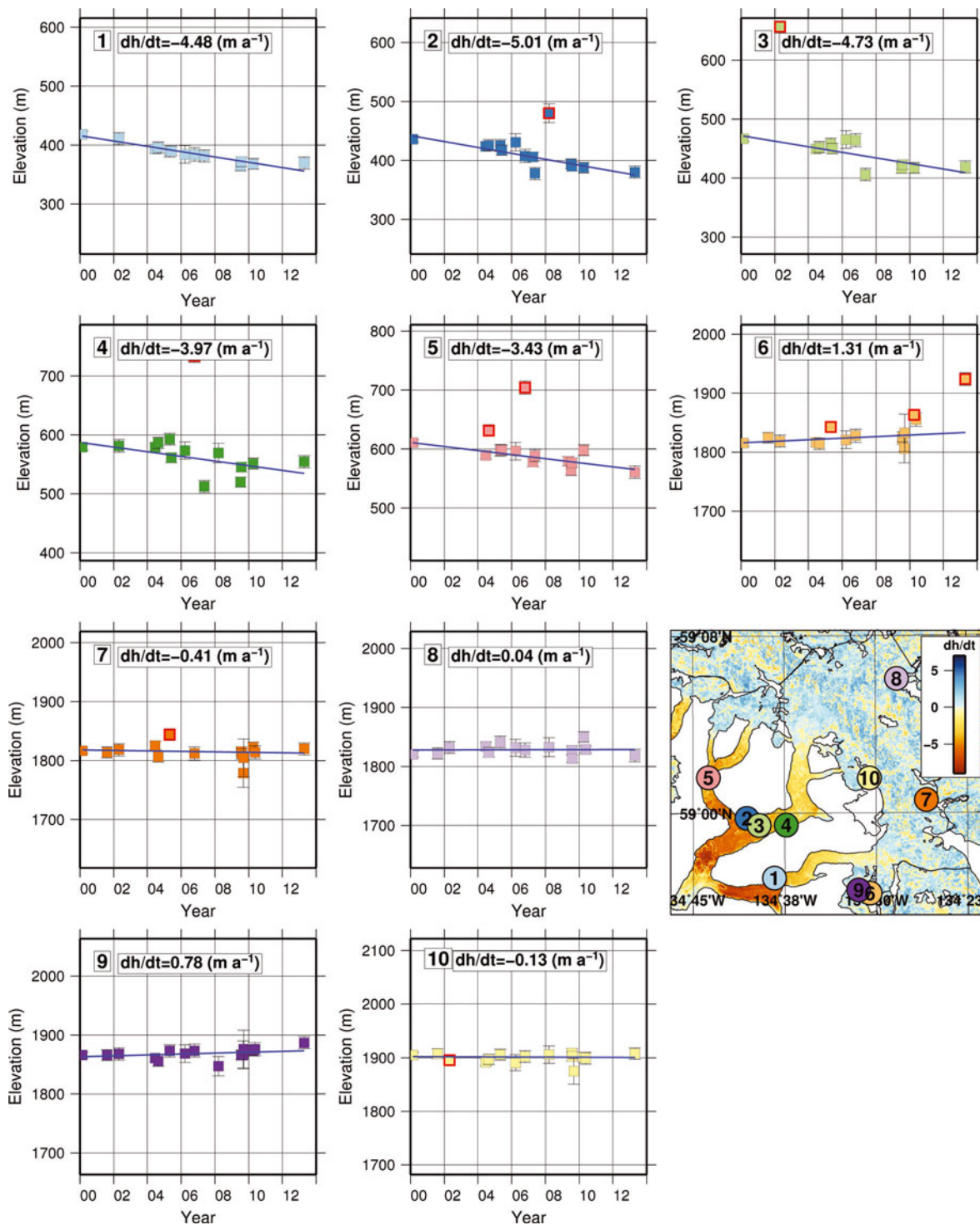
Fig. 4. Elevation values and \frac{dh}{dt} for randomly selected pixels over Field Glacier. The leftmost elevation in each graph is the SRTM elevation at that pixel. Blue lines indicate the \frac{dh}{dt} calculated for each pixel. Elevation points bolded red are excluded from \frac{dh}{dt} calculation. The bottom right panel shows the \frac{dh}{dt} map (location in Fig. 5), with numbered circles indicating the location corresponding to each graph.
