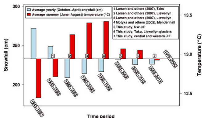
Fig. 8. Total winter (October–April) snowfall (cm) in blue, and average summer (June–August) temperature ( ^{\circ}\text{C} ) in red, for study periods spanning 1948–2013, shown as deviations from the 1970–2000 averages (horizontal black line). Data are from the Juneau International Airport station.
