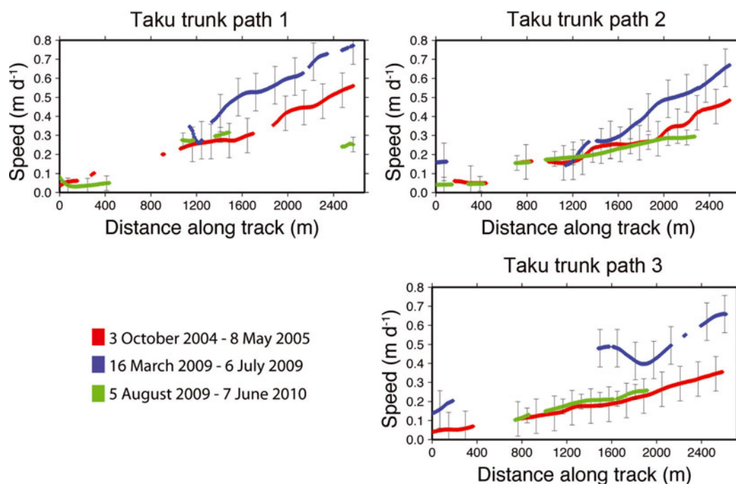
Fig. 14. Speeds along tracks 1, 2 and 3 (see Fig. 13) for ASTER image pairs October 2004 to May 2005 (red), March 2009 to July 2009 (blue) and August 2009 to June 2010 (green). Uncertainties ( \mu \pm \sigma ) represented as gray bars. All speeds increase with distance from the front, ranging from about 0.05 to 0.7 \text{m d}^{-1} . ‘Summer’ speeds (March 2009 to July 2009) are higher than speeds for the other pairs, especially for track 3 (the southwestern track).
