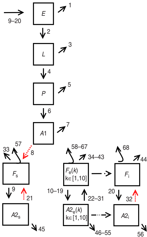
Fig. 1 [colour online]. Mosquito dynamics. Subpopulations and events of the stochastic model according to Table 1.
