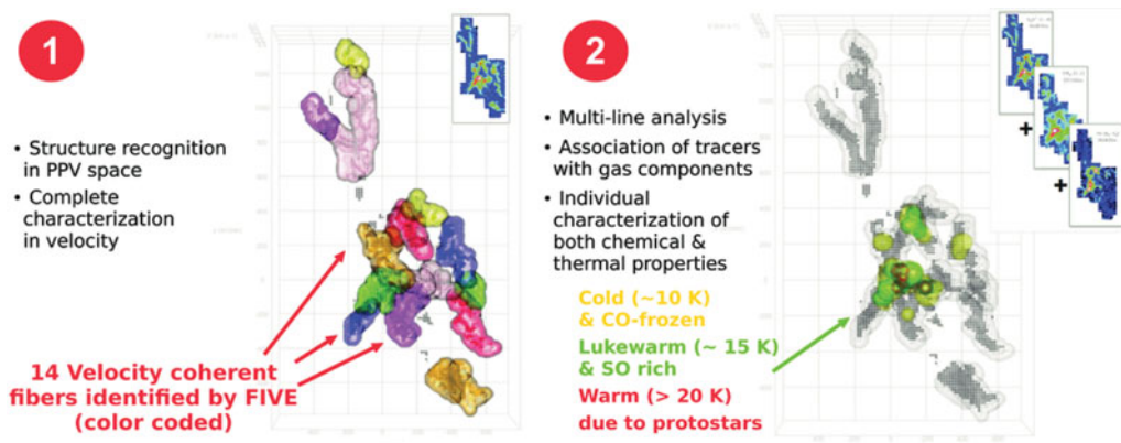
Figure 1. Preliminary FIVE+ results in the NGC1333 proto-cluster. (Left) 14 velocity-coherent fibers identified in the PPV space in \text{N}_2\text{H}^+ (color coded; Hacar et al. 2013). A full visualization of these results can be found in https://sites.google.com/site/orion4dproject/visualization . (Right) New multi-line FIVE+ analysis combining the information of all \text{N}_2\text{H}^+ (1-0), \text{NH}_3 (1,1) & (2,2), and SO ( 6_5-5_4 ) tracers within the same region. This joint analysis makes possible to systematically characterize the gas density ( \text{N}_2\text{H}^+ ; grey structures), gas temperature (SO + \text{NH}_3 ; red and green regions), and chemical compositions of each individual structure both in position and velocity (see PPV iso-surfaces).
