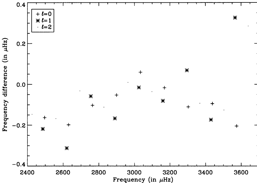
Figure 1. Frequency difference between BiSON and LOI for l = 0 - 2 as a function of frequency. The typical error bar on the measurement of a single mode frequency ranges from 0.10 \mu\text{Hz} to 0.15 \mu\text{Hz} .
