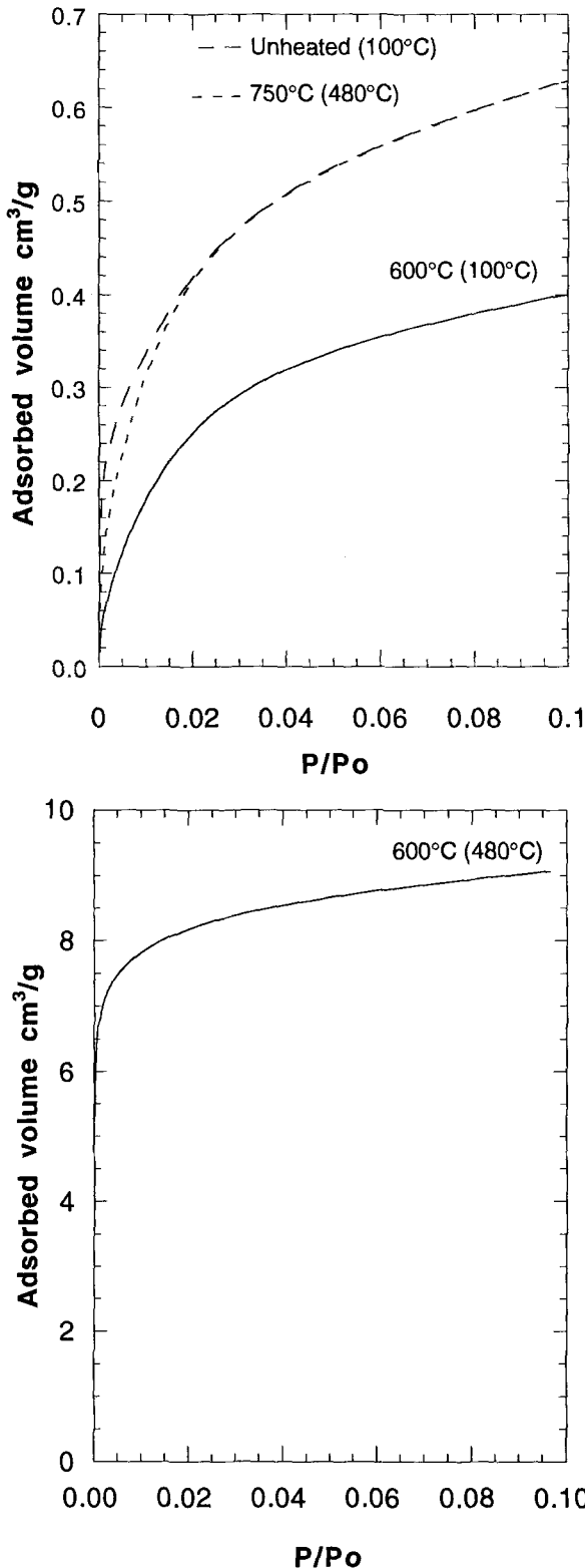
Figure 9. Argon adsorption isotherms at 77 K on chlorite M heated and outgassed in various conditions. The first value corresponds to the heating temperature, the value in brackets indicates the outgassing temperature.
