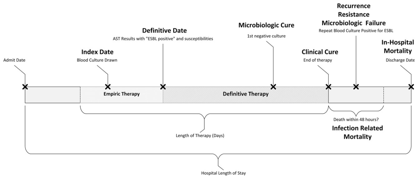
Fig 1. Definitions timeline.
