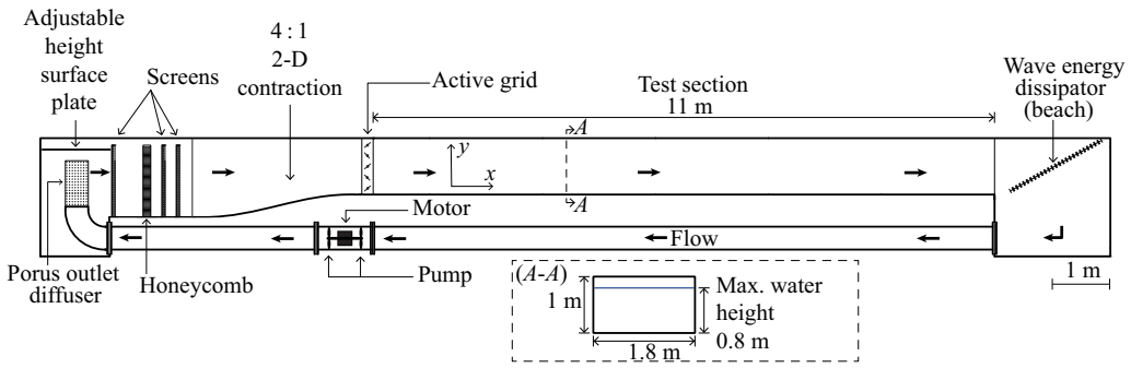
FIGURE 1. Schematic of the water channel facility in Strømningslaben at the Norwegian University of Science and Technology.
