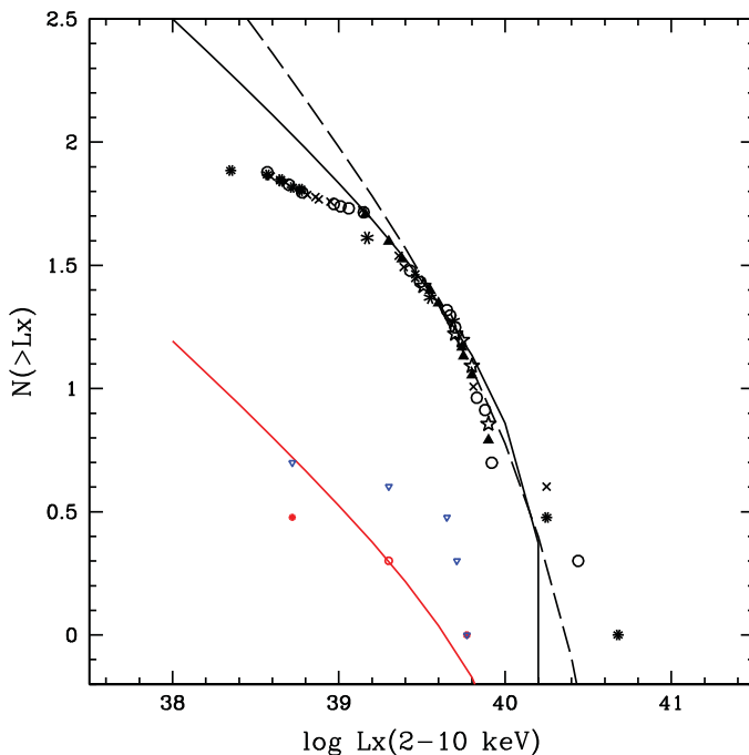
Figure 5. The total X-ray luminosity function (XLF) derived from the 6 observed ring galaxies (see text). The black solid line is the model of Grimm et al. (2003), normalized to SFR = 61 M_{\odot} \text{ yr}^{-1} , which is the sum of the SFR for the 6 “pointed” galaxies. The dashed line is the XLF from Swartz et al. (2011). In this plot, we consider only the sources associated to the rings. There are 50 sources in total, and 15 sources above L_X > 5 \times 10^{39} \text{ erg s}^{-1} . Different symbols correspond to the different galaxies. Four sources are about the cut-off limit and have L_X(2-10 \text{ keV}) > 10^{40} \text{ erg/s} . The red(blue) points are secure(all) sources from the “statistical” sample. The red solid line is the Grimm et al. (2003) model rescaled to SFR = 3 M_{\odot} \text{ yr}^{-1} .
