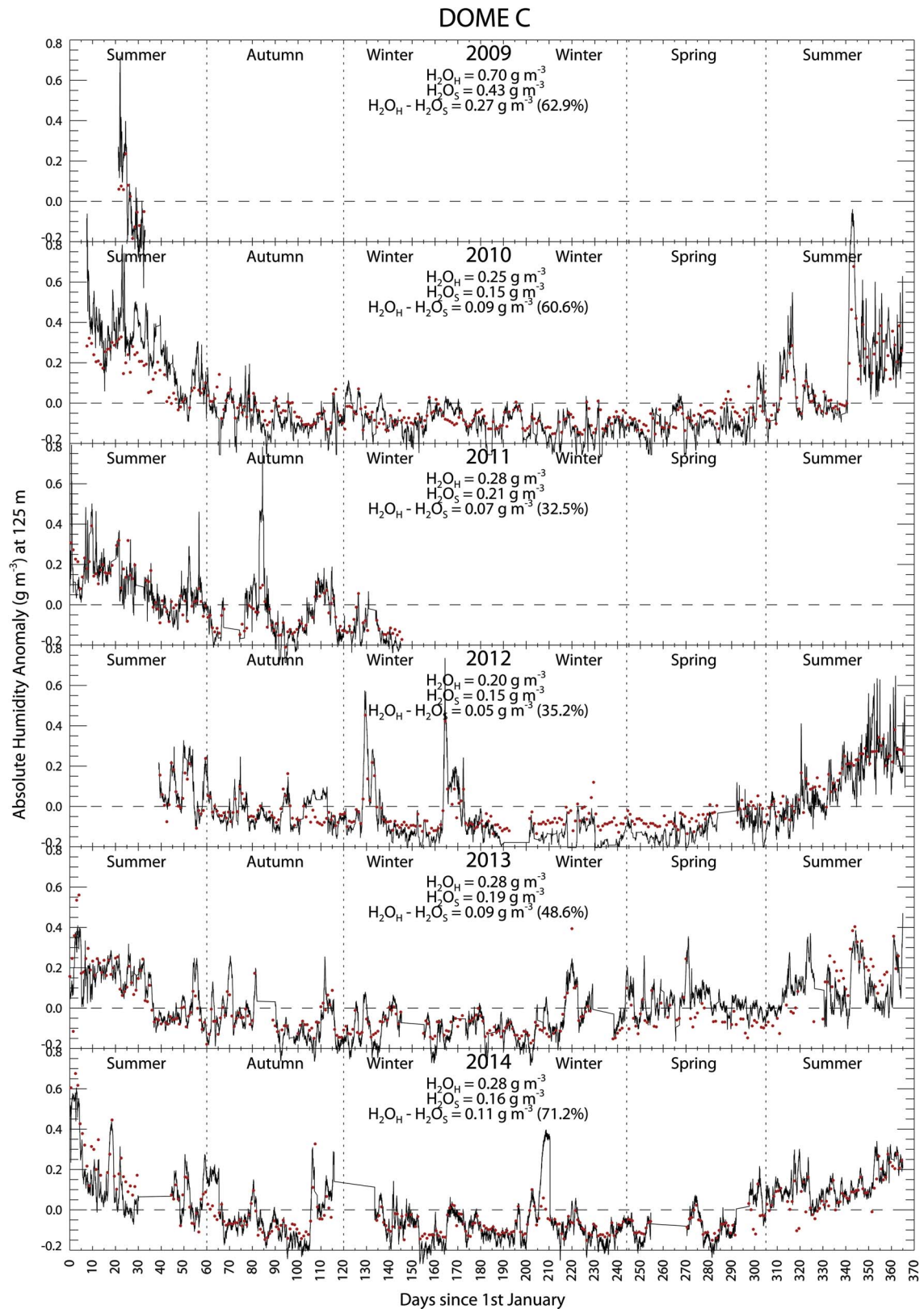
Fig. 9. Time series from 2009 to 2014 (top to bottom) of the absolute humidity anomaly ( g\ m^{-3} ) at 125 m as measured by HAMSTRAD (black line) and the radiosondes (red dots). The yearly-averaged absolute humidity ( g\ m^{-3} ) from HAMSTRAD ( H_2O_H ) and from the radiosondes ( H_2O_S ) and the difference ( H_2O_H - H_2O_S ) are highlighted in each panel, together with the relative difference (%).
