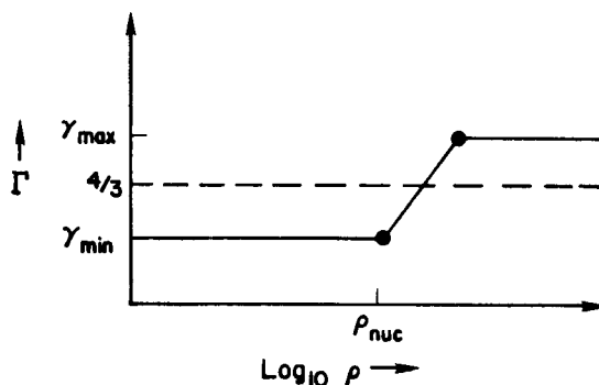
Fig. 1. The function \Gamma(\rho) used to define the adiabatic collapse
