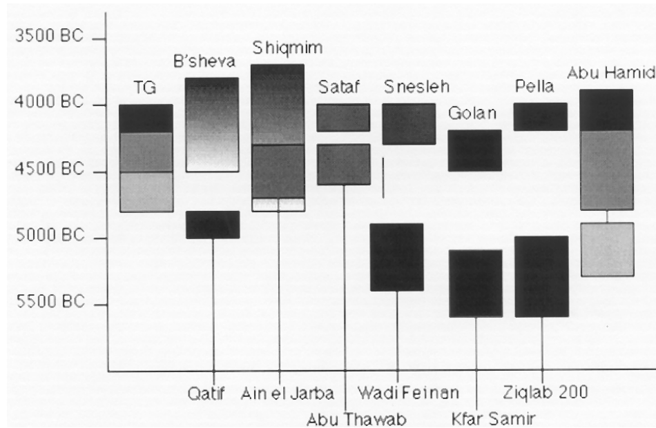
Figure 2 Revised relative chronology for southern Levantine Chalcolithic assemblages
