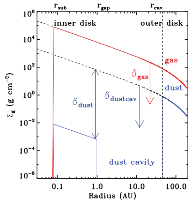
Figure 3. Generic surface density model of gas and dust that is used as input for DALI. Inside the cavity ( < r_{\text{cav}} ), the dust density drops by a factor \delta_{\text{dustcav}} , the gas density by a factor \delta_{\text{gas}} . The inner disk is reproduced by an additional \delta_{\text{dust}} . The \delta -values are free parameters in the model, after the outer disk density is matched to the data. Figure taken from van der Marel et al. (2015a).
