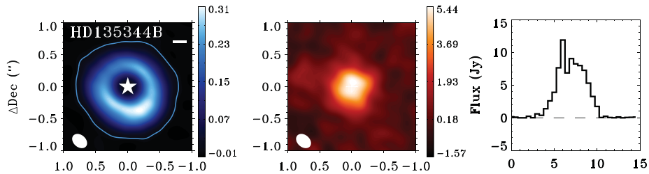
Figure 1. ALMA observations of the 690 GHz dust continuum and ^{12}\text{CO} 6-5 line of HD135344B, one of six targets in the sample of the ^{12}\text{CO} study in van der Marel et al. (2015a). In the images, the beam is indicated in the lower left corner. Left: Continuum image. The white bar in the upper right corner indicates the 30 AU scale and the yellow contour gives the 3\sigma detection limit. Center: zero-moment ^{12}\text{CO} map. Right: ^{12}\text{CO} spectrum integrated over the entire disk. The dashed line indicates the zero flux level.
