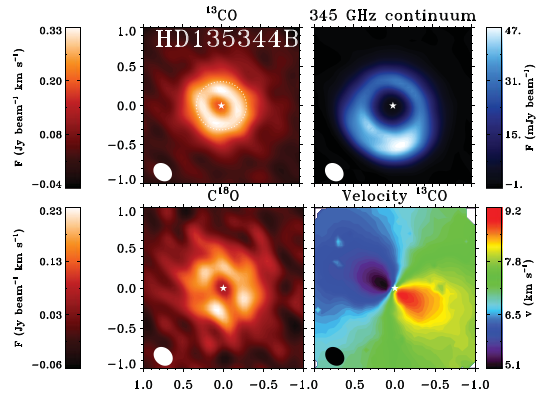
Figure 4. ALMA Cycle 1 observations of the continuum, ^{13}\text{CO} and \text{C}^{18}\text{O} 3-2 lines of HD135344B. Top left: zero-moment ^{13}\text{CO} map; Top right: Continuum map; Bottom left: zero-moment \text{C}^{18}\text{O} map; Bottom right: first moment ^{13}\text{CO} map.
