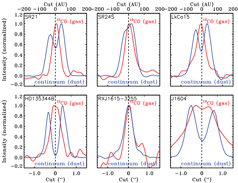
Figure 2. Normalized intensity cuts along the major axis of the continuum emission and the integrated ^{12}\text{CO} map of each disk in the sample. The continuum is indicated in blue, the integrated ^{12}\text{CO} in red. The cuts reveal that the ^{12}\text{CO} emission is peaking inside the dust cavity.
