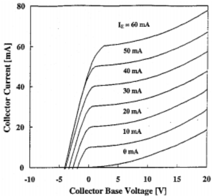
Figure 7. Common base I-V characteristics at 520
