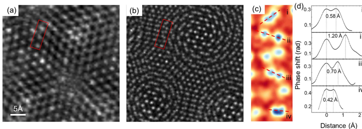
Figure 2. Real-space resolution demonstration of full-field ptychography using a twisted bilayer MoS 2 . (a) Synthesized ADF image; (b) Phase image from ptychographic reconstruction of the same region as (a); (c) Enlarged phase image of the marked area in (b); (d) Intensity line profile of corresponding positions labeled with dashed red lines in (c). The peak separation distances are labelled in (d).
