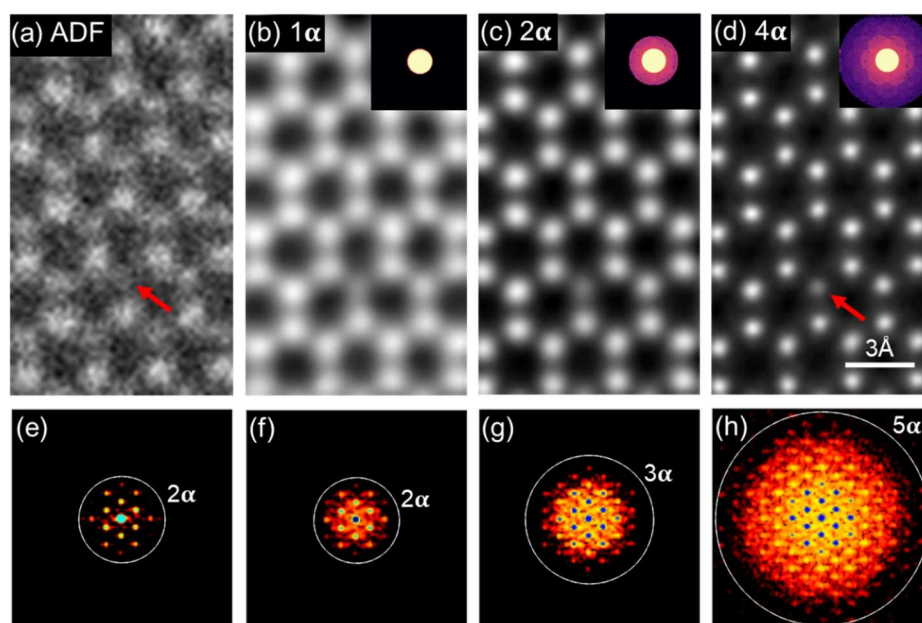
Figure 1. Resolution improvement of ptychographic reconstructions of monolayer MoS 2 with increasing collection angle. (a) Synthesized ADF image from the same EMPAD dataset. Ptychographic reconstructions applying different cutoffs: (b) only the central bright field disk (1 \alpha ), (c) up to 2 \alpha , and (d) up to 4 \alpha . (e)-(h) Diffractograms corresponding to (a)-(d) with white circles showing the information limit. 5 \alpha corresponds to a 0.39 Å Abbe resolution. The red arrows point out a sulfur mono-vacancy.
