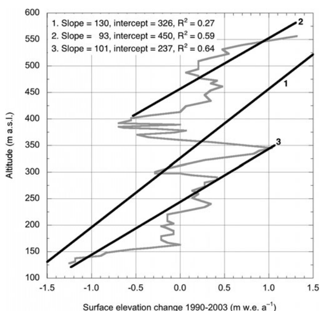
Fig. 4. Surface elevation with altitude. Linear regression 1 is significant with 95% probability, though weak. Regressions 2 and 3 achieve much better fits with the same probability, by excluding the altitude interval 350–400 m a.s.l., the steepest part of the glacier with a locally negative elevation-change gradient (see Fig. 3).
