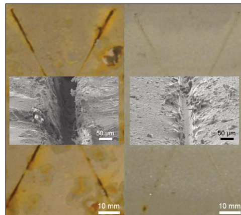
Figure 1. The background images show the dramatic reduction in corrosion of steel plates coated with a self-healing coating (right) as compared to a conventional coating (left) after they were both scratched and subsequently immersed in 5% salt (NaCl) water for five days. The foreground pictures are scanning electron microscope images of the control (left) and healed (right) scratch showing the repair of the scratch in the self-healing coating.
