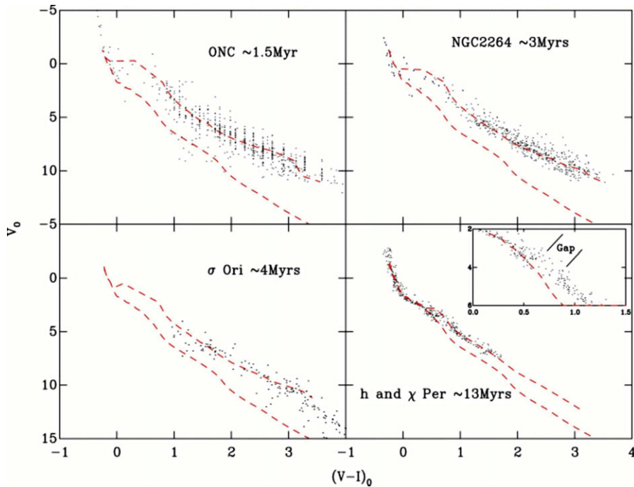
Figure 1. The CMDs for a selection of young groups in absolute magnitude and intrinsic colour. In each case the lower red dotted line is the position of the MS, the upper an appropriate Siess et al. (2000) isochrone.
