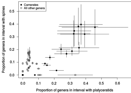
FIGURE 5. Proportion of crinoid genera hosting platyoceratid gastropod epibionts vs. proportion with spines in each time interval for the Paleozoic, with camerates and non-camerates separated. Error bars indicate \pm 1 SE. The proportion of spiny genera and that of infested genera are well correlated for camerates, but no relationship between spinosity and infestation is evident for any other taxon.
