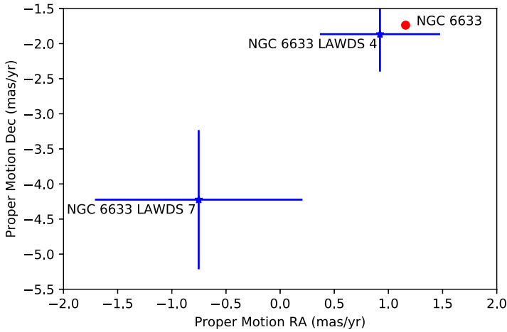
Figure 1. Gaia DR2 proper motion data for NGC 6633 and the two candidate double degenerates, with 1\sigma error bars. The uncertainties and dispersions for the cluster are smaller than the data point. This plot shows that the proper motions of LAWDS 4 are consistent with cluster membership, while LAWDS 7 appears to be inconsistent.
