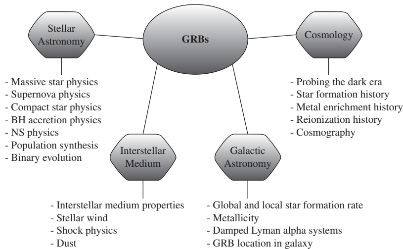
Figure 1.2 A flowchart showing connections between the GRB field and other major branches in astrophysics. Figure courtesy Jared Rice.
