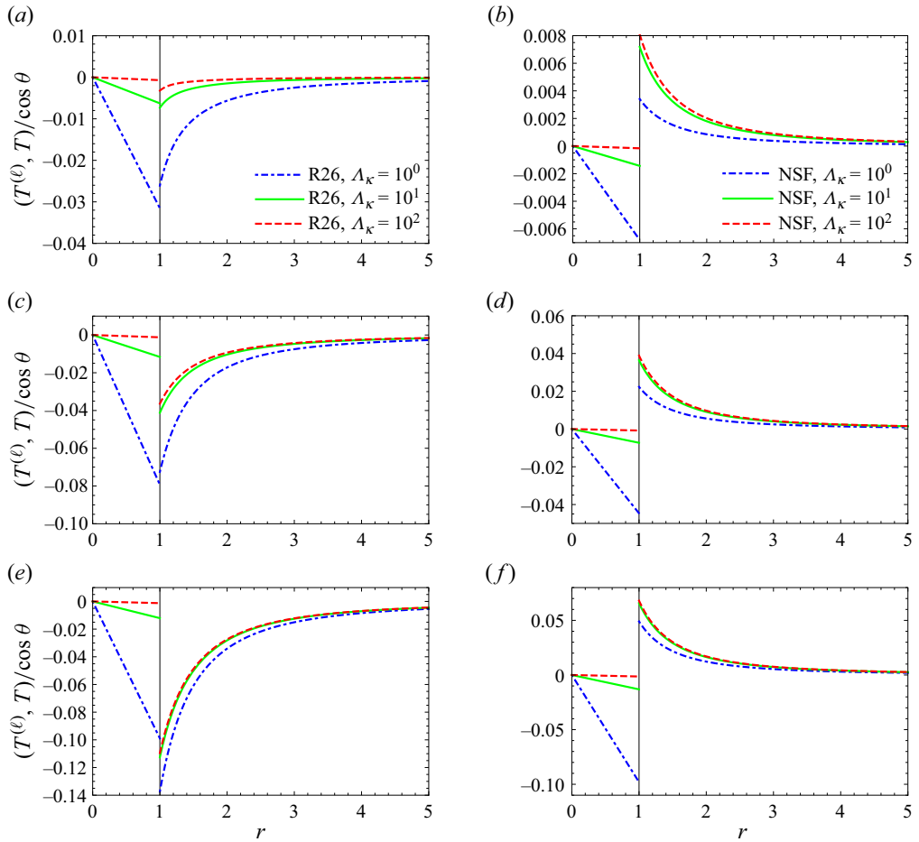
Figure 7. Dimensionless deviations in the temperature (scaled with \cos \theta ) as a function of position r for a fixed viscosity ratio \Lambda_\mu = 100 and for different values of the Knudsen number: Kn = 0.09 (a,b), Kn = 0.36 (c,d) and Kn = 0.9 (e,f). The vertical black line at r = 1 demarcates the interface between the liquid and gas. The results for the liquid phase (internal flow) have been computed with the NSF equations in all the cases while those for the gas phase (external flow) have been computed with the LR26 equations (a,c,e) and with the NSF equations (b,d,f).
