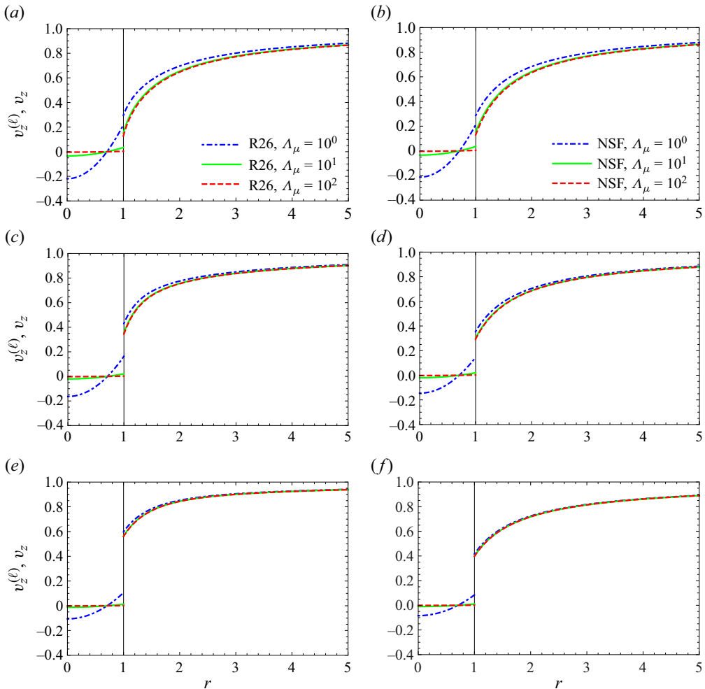
Figure 13. The z -component of the (dimensionless) velocity as a function of position r in the plane \theta = \pi/2 for a fixed thermal conductivity ratio \Lambda_\kappa = 100 and for different values of the Knudsen number: Kn = 0.09 (a,b), Kn = 0.36 (c,d) and Kn = 0.9 (e,f). The vertical black line at r = 1 demarcates the interface between the liquid and gas. The results for the liquid phase (internal flow) have been computed with the NSF equations in all the cases while those for the gas phase (external flow) have been computed with the LR26 equations (a,c,e) and with the NSF equations (b,d,f).
