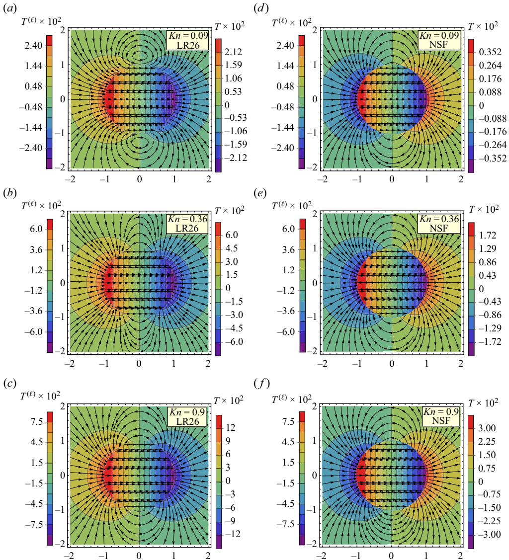
Figure 4. Heat flux lines plotted on top of the temperature contours for the viscosity ratio \Lambda_\mu = 100 and for different values of the Knudsen number: Kn = 0.09 (a,d), Kn = 0.36 (b,e) and Kn = 0.9 (c,f). The results for the liquid phase (internal flow) have been computed with the linear NSF equations in all the cases while those for the gas phase (external flow) have been computed with the LR26 equations (a–c) and with the linear NSF equations (d–f). The thermal conductivity ratio is \Lambda_\kappa = 1 .
