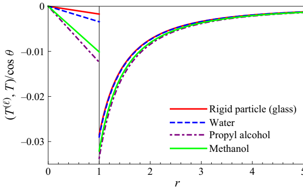
Figure 14. Dimensionless deviations in the temperature (scaled with \cos \theta ) as a function of position r for Kn = 0.3 in the case of argon gas flow past a rigid spherical glass ball (solid red lines), in the cases of argon gas flow past spherical liquid droplets of water (dashed blue lines), propyl alcohol (purple dot–dashed lines) and methanol (green solid lines). The vertical black line at r = 1 demarcates the interface between the solid/liquid and gas.
