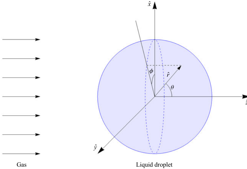
Figure 1. Schematic of a rarefied gas flow past a spherical liquid droplet.
