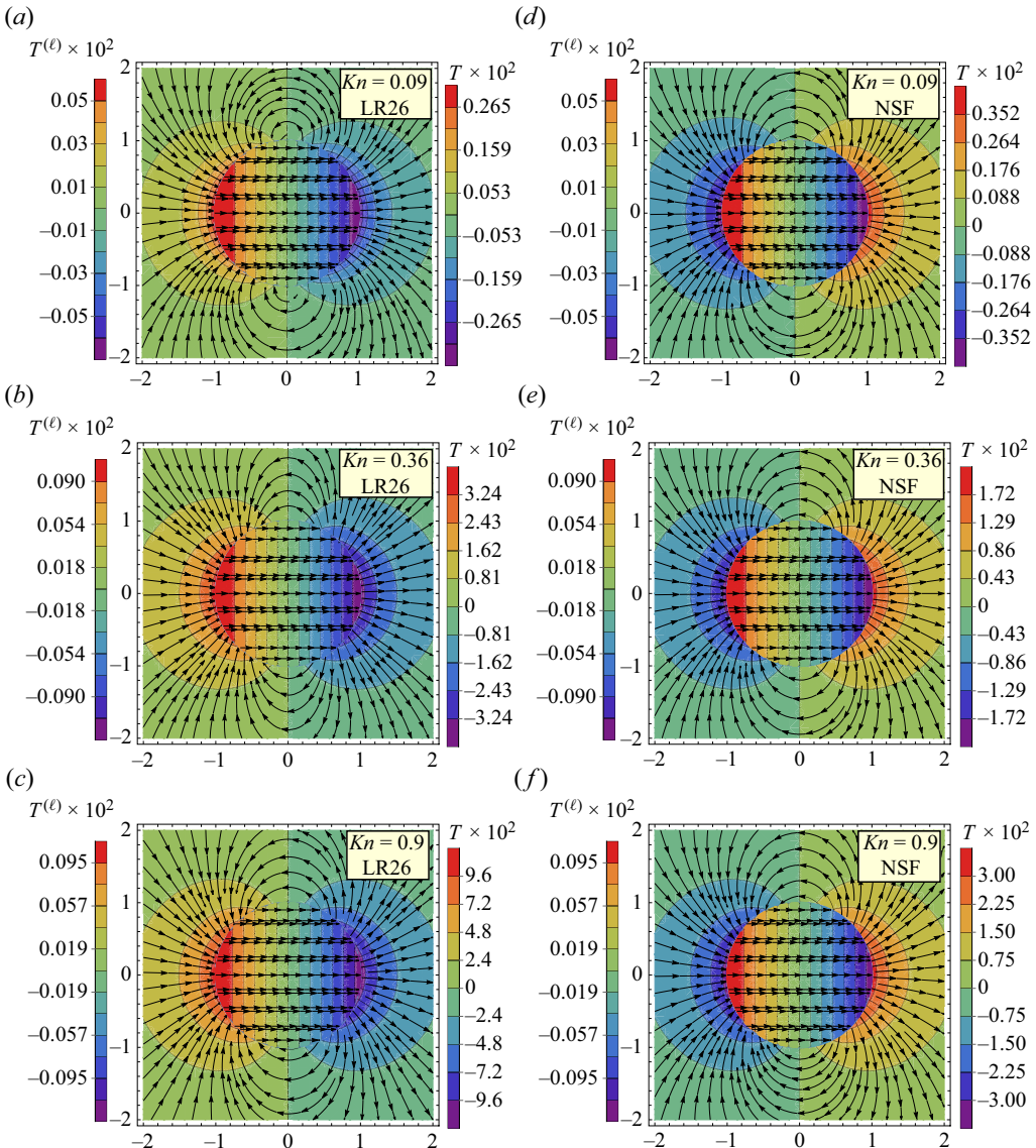
Figure 6. Same as figure 4 but for the thermal conductivity ratio \Lambda_\kappa = 100 .
