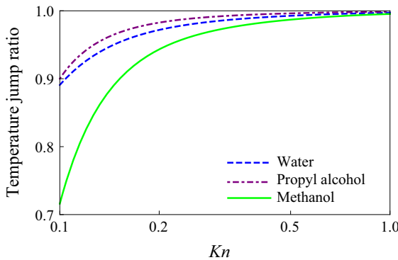
Figure 15. The ratio of the temperature jump at the interface of a liquid droplet (made of water, propyl alcohol and methanol) to the temperature jump at the interface of a corresponding solid sphere ( \Lambda_\mu \rightarrow \infty ) having the same thermal conductivity as that of the liquid against plotted over the Knudsen number.
