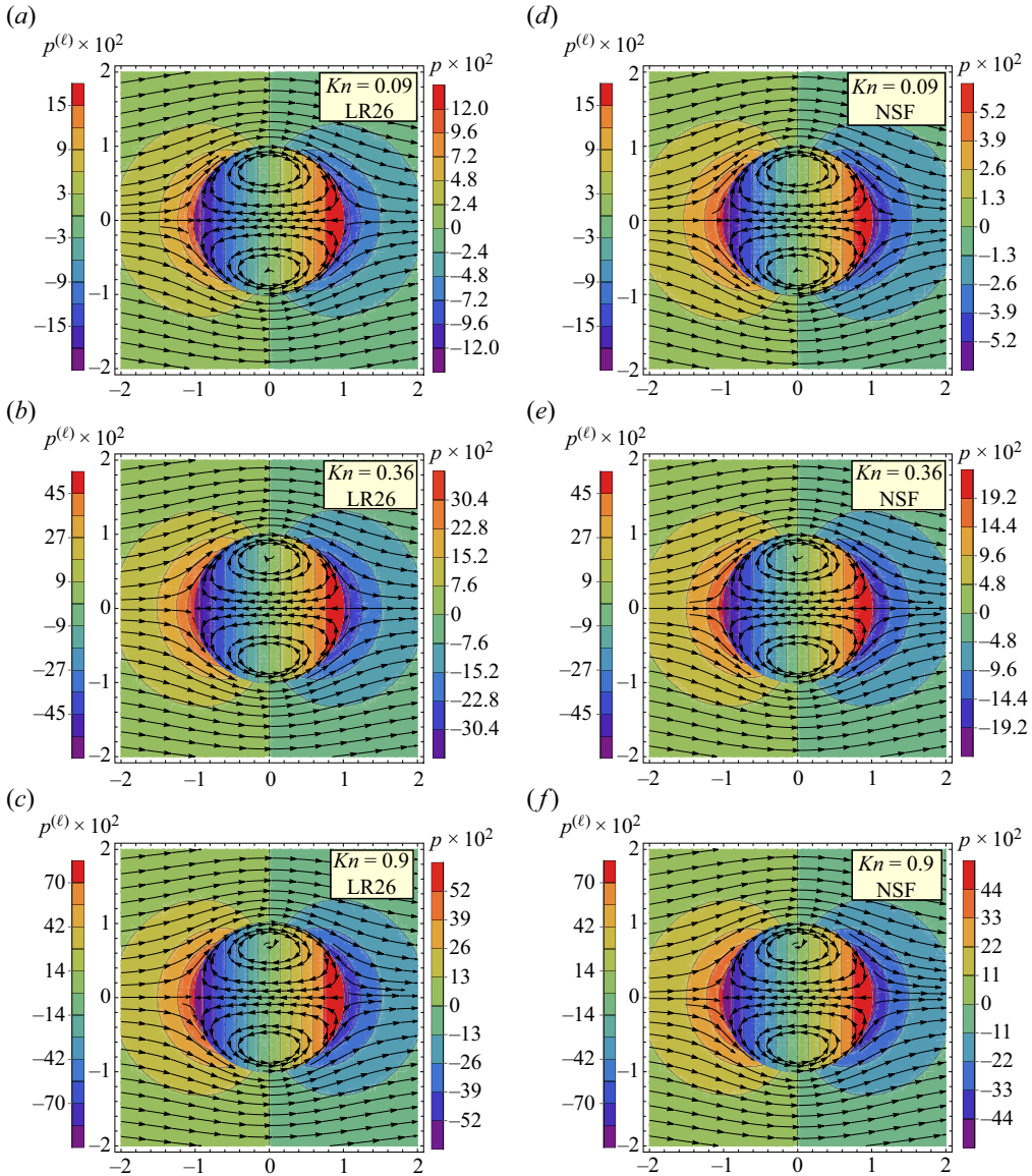
Figure 9. Velocity streamlines plotted over the pressure contours for the thermal conductivity ratio \Lambda_\kappa = 100 and for different values of the Knudsen number: Kn = 0.09 (a,d), Kn = 0.36 (b,e) and Kn = 0.9 (c,f). The results for the liquid phase (internal flow) have been computed with the NSF equations in all the cases while those for the gas phase (external flow) have been computed with the LR26 equations (a–c) and with the NSF equations (d–f). The viscosity ratio is \Lambda_\mu = 1 .
