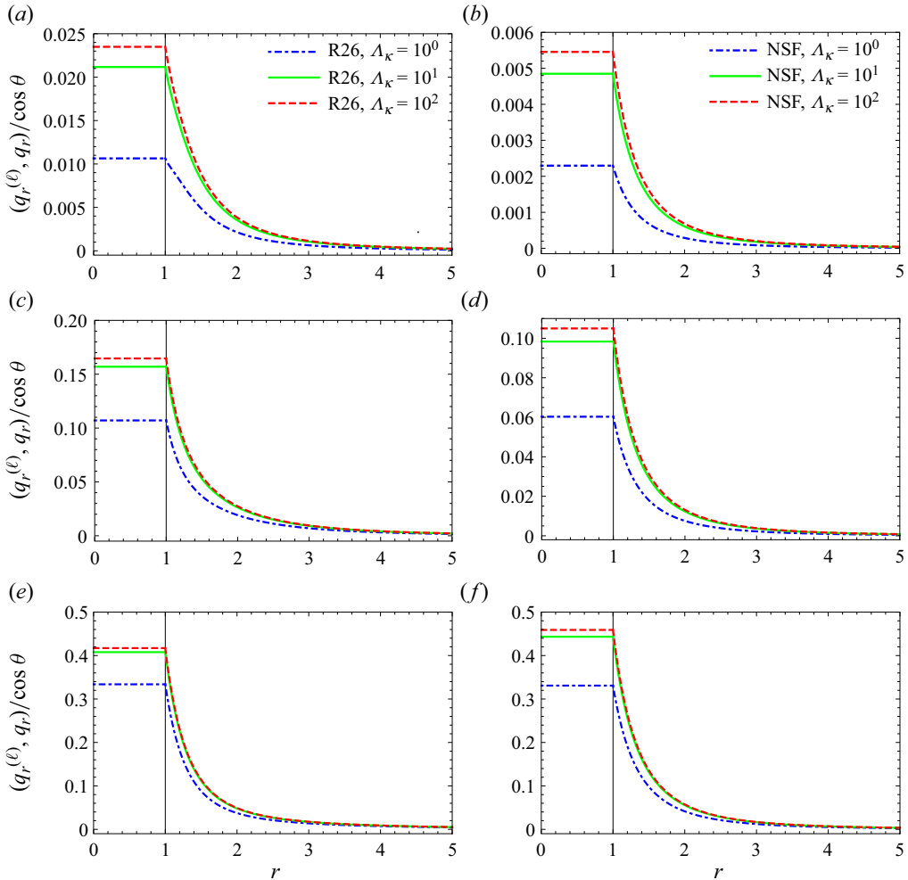
Figure 8. Dimensionless radial heat flux (scaled with \cos \theta ) as a function of position r for a fixed viscosity ratio \Lambda_\mu = 100 and for different values of the Knudsen number: Kn = 0.09 (a,b), Kn = 0.36 (c,d) and Kn = 0.9 (e,f). The vertical black line at r = 1 demarcates the interface between the liquid and gas. The results for the liquid phase (internal flow) have been computed with the NSF equations in all the cases while those for the gas phase (external flow) have been computed with the LR26 equations (a,c,e) and with the NSF equations (b,d,f).
