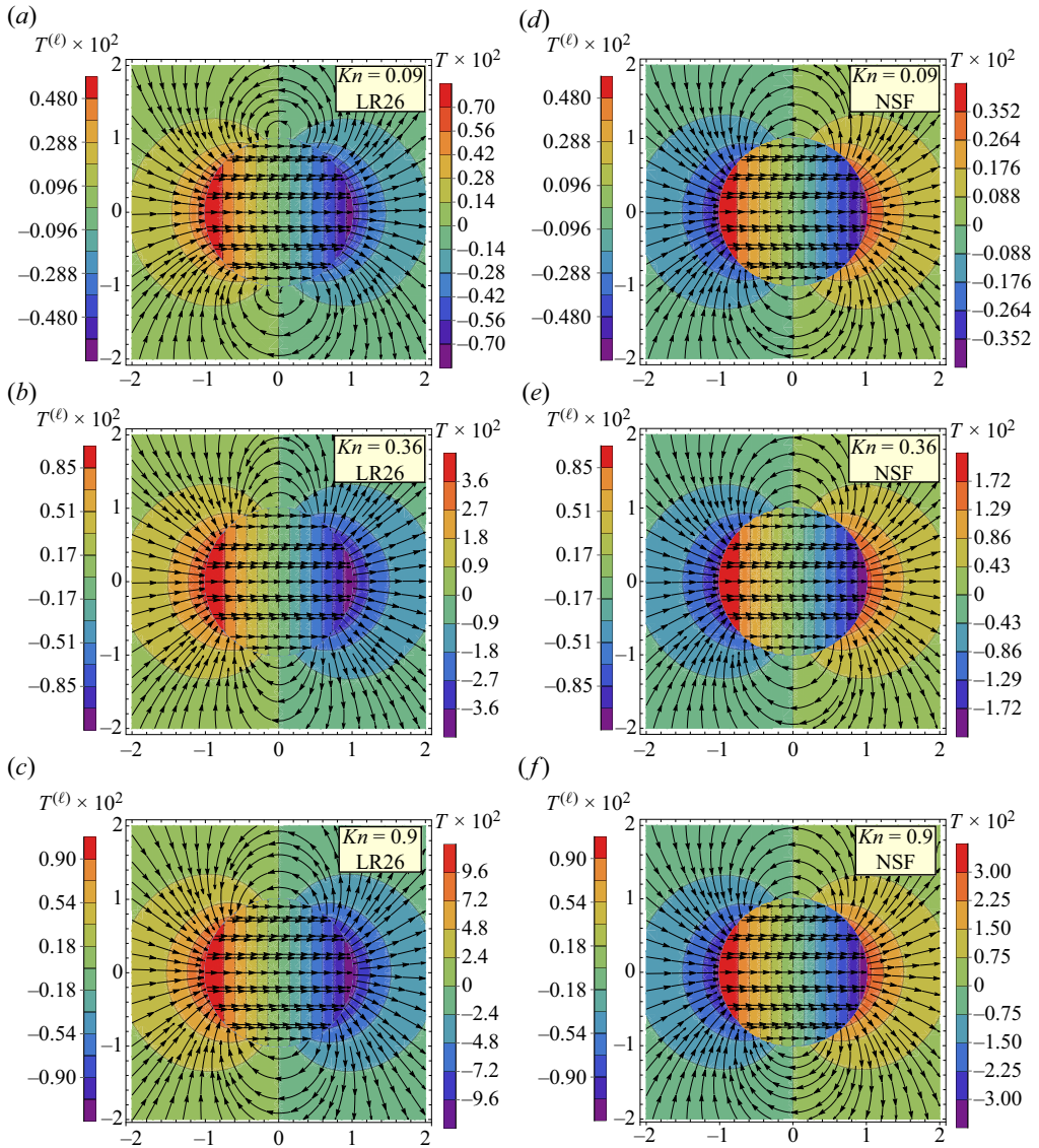
Figure 5. Same as figure 4 but for the thermal conductivity ratio \Lambda_\kappa = 10 .
