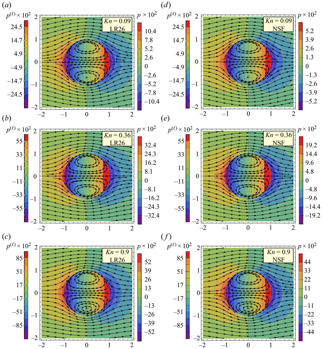
Figure 11. Same as figure 9 but for the viscosity ratio \Lambda_\mu = 100 .
