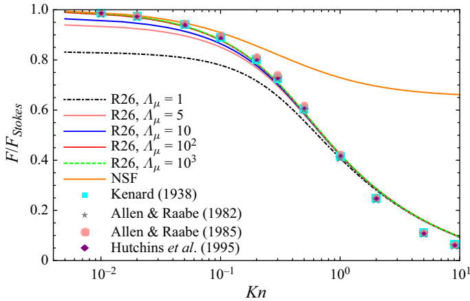
Figure 2. Drag force (normalised with the Stokes drag F_{Stokes} = 6\pi Kn u_\infty ) on a liquid droplet from the linearised NSF and R26 theories as a function of the Knudsen number for a fixed thermal conductivity ratio \Lambda_\kappa = 100 . The square and star symbols denote the experimental data from Millikan’s oil-drop experiment fitted by the empirical formulae of Kennard (1938) ((4.1) with (4.2a–c)) and Allen & Raabe (1982) ((4.1) with (4.2a–c)), respectively. The disk and diamond symbols denote the data from experiments performed with solid spherical particles in air fitted by the empirical formulae of Allen & Raabe (1985) ((4.1) with (4.2a–c)) and Hutchins et al. (1995) ((4.1) with (4.2a–c)), respectively, and are included just for comparison.
