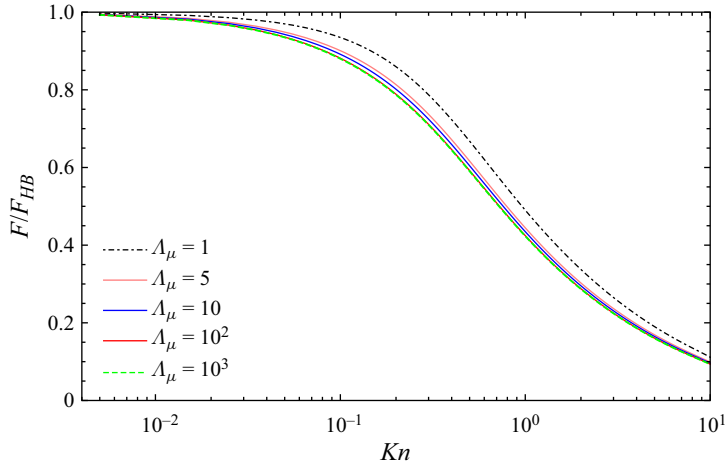
Figure 3. Drag force on the liquid droplet normalised with the drag force given by (4.9). The thermal conductivity ratio is \Lambda_\kappa = 100 .
