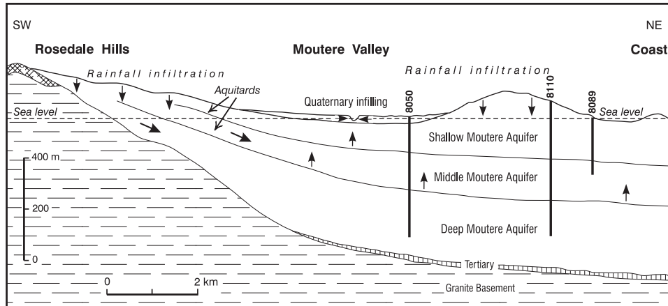
Figure 2 Cross-section showing the structure of the basin underlying the Moutere Catchment. The trace of the cross-section is parallel to the fault in Figure 1b. Inferred recharge patterns for the Moutere aquifers are shown (Stewart and Thomas 2002).
