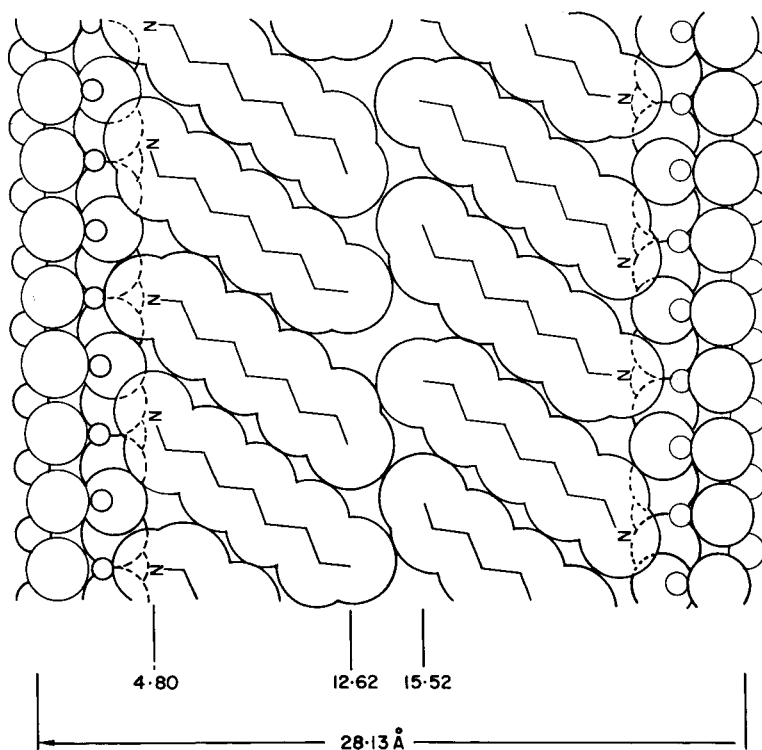
Fig. 2. Structure of the octyl-ammonium-vermiculite complex (fully expanded phase, 28.1 Å) after Johns and Sen Gupta (1967).
