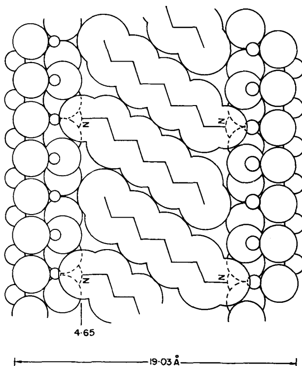
Fig. 1. Structure of the octyl-ammonium-vermiculite complex (collapsed phase, 19·0 Å) after Johns and Sen Gupta (1967).
