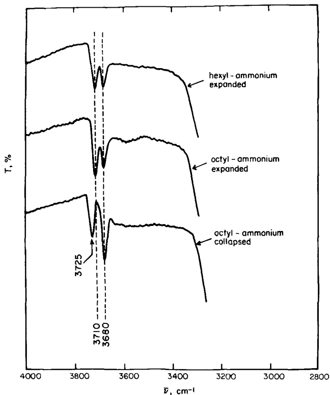
Fig. 6. I.R. spectra of octyl-ammonium complexes in the OH region for inclined incidence ( 40^\circ ). The two observed frequencies represent the unperturbed ( 3680\text{ cm}^{-1} ) and perturbed (high frequency) structural OH groups. The spectrum of the fully expanded hexyl-ammonium complex is included for comparison.
