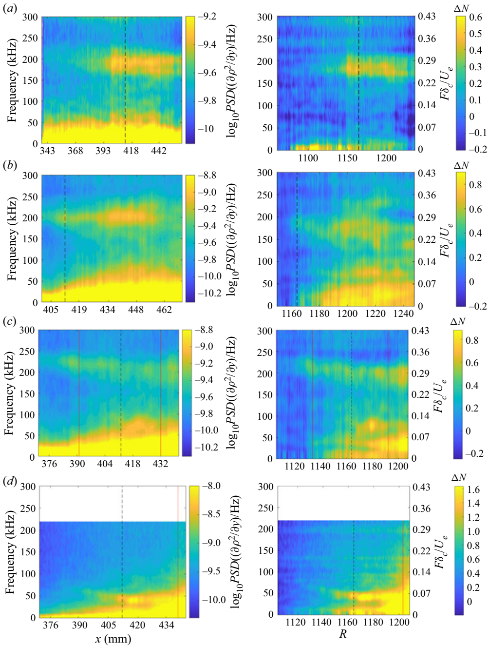
Figure 14. Power spectral densities (left panels) and N -factor distributions (right panels) computed along pseudo-streamlines at condition Re33 for the (a) +0°, (b) +5°, (c) +10° and (d) +15° configurations. The dashed and solid vertical lines indicate corner and (where relevant) separation/reattachment locations.
