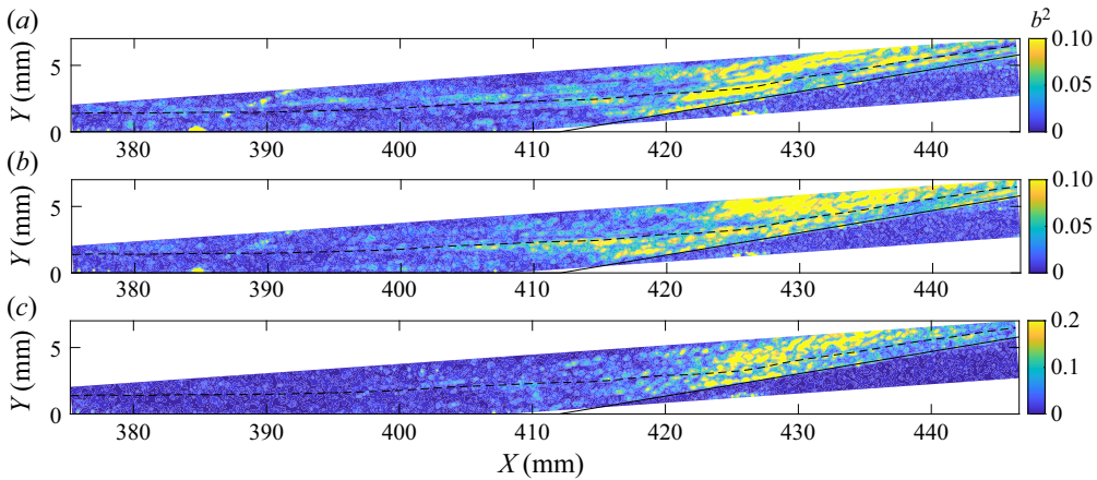
Figure 39. Spatial bicoherence contours for the +10° flare at condition Re45 for frequency triplets of (a): [55,55,110], (b) [75,75,150] and (c) [160,160,320].
