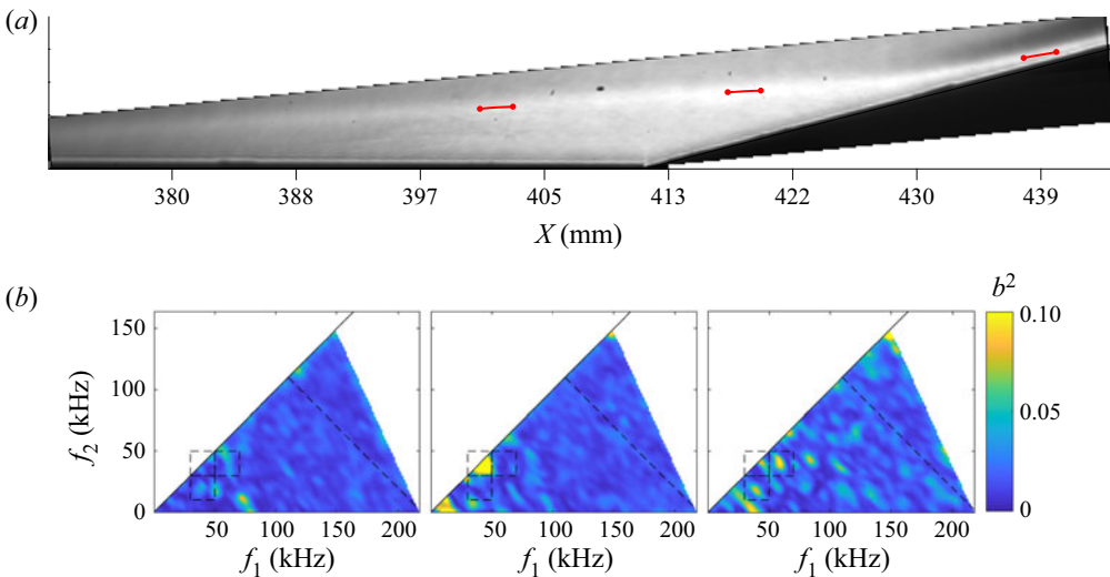
Figure 40. As in figure 32 but for the +15° configuration at condition Re33.
