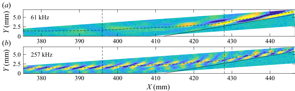
Figure 28. The SPOD mode shapes for the +10^\circ configuration at condition Re45 at (a) 61 kHz and (b) 257 kHz.
