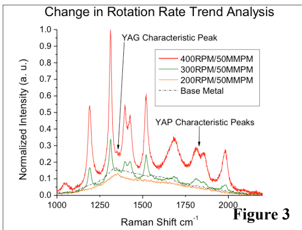
Figure 3. Systematic change in Raman spectra as a function of increasing FSW tool rotation speed.
