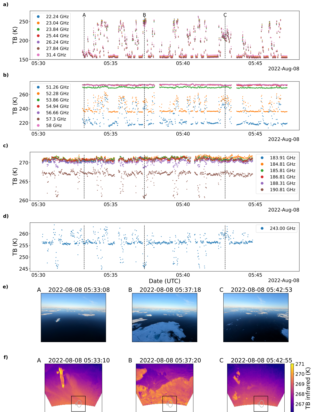
Fig. 6. Same as Fig. 5 but for 8 August 2022, 5:30 to 5:47 UTC.
