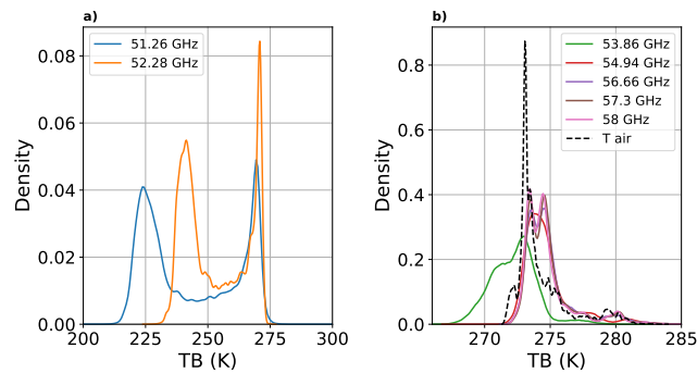
Fig. 8. All surface TB observations during ATWAICE at frequencies (a) 51.26 and 52.28 GHz and (b) between 53.86 to 58 GHz at a 53^\circ zenith angle and predominantly-horizontal polarization. The total number of measurements is 485,649 (equivalent to about 135 hours). The data is shown as probability density using kernel density estimation with a Gaussian kernel. In addition the distribution of air temperatures ( T_{\text{air}} ) measured onboard is shown (dashed black line).
