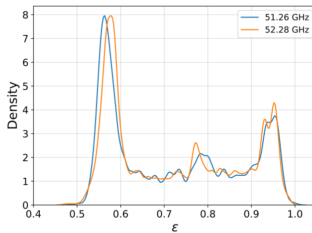
Fig. 15. Kernel density estimate of the distribution of emissivities ( \epsilon ) calculated for the frequencies 51.26 and 52.28 GHz at a 53^\circ zenith angle for manually selected times with clear sky (N=3730).
