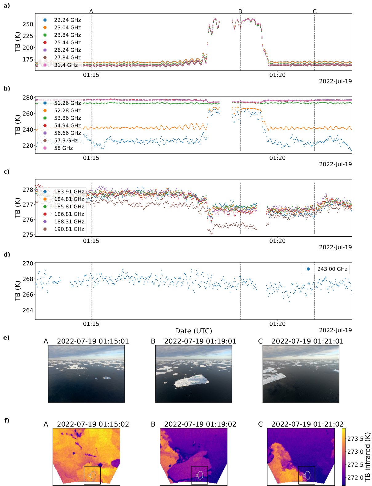
Fig. 12. Same as Fig. 5 but for 19 July 2022, 01:13 to 01:22 UTC.
