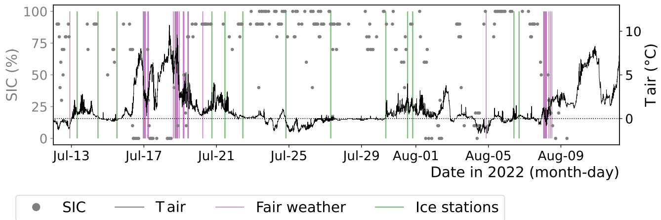
Fig. 2. Time series of sea ice concentration (SIC), air temperature ( T_{air} , secondary axis), fair weather intervals, and occurrence of ice stations from 12 July to 12 August 2022. The sea ice concentration is estimated in steps of 10% until 9 August 2022.
