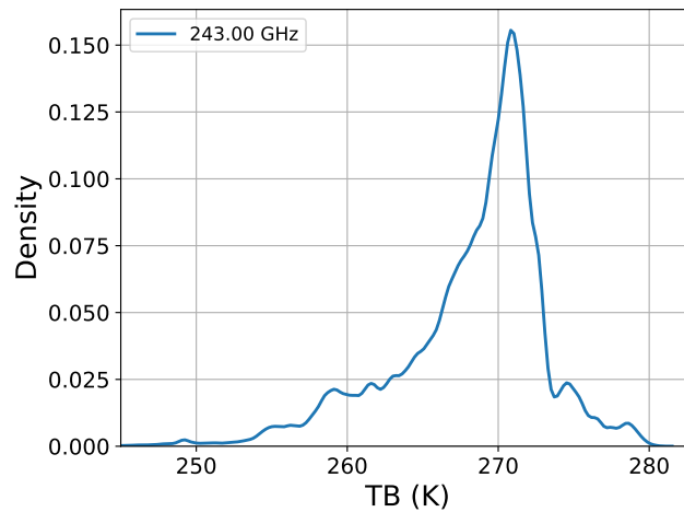
Fig. 10. Same as Fig. 7 but for 243 GHz, predominantly-horizontal polarization. The total number of measurements is 600,607 (equivalent to about 167 hours).
