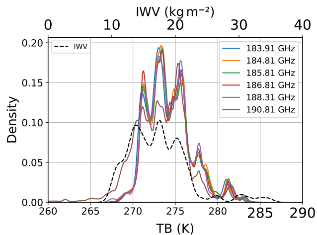
Fig. 9. All surface TB observations during ATWAICE at frequencies in the 183 GHz water vapor line at a 53^\circ zenith angle and predominantly-vertical polarization. The total number of measurements is 600,607 (equivalent to about 167 hours). The data is shown as probability density using kernel density estimation with a Gaussian kernel. In addition the distribution of integrated water vapor (IWV) derived from 117 radiosonde measurements is shown (dashed black line).
