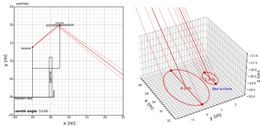
Fig. 4. Mirror setup. Left: The receiver of the radiometer is positioned at x=0\text{ m} with an elevation angle of 40^\circ . Because of the mirror alignment, this results in a zenith angle of 53^\circ . The mirror has a size of 0.55\text{ m}^2 . The red lines are the path of rays of the microwave radiation with the center and the outer rays obtained from the beam width (3dB). Right: projected footprints of HATPRO (left ellipse) and MiRAC-P (right ellipse) on the surface.
