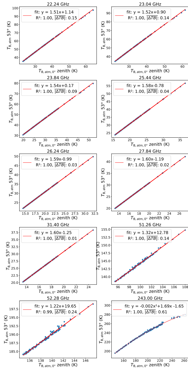
Fig. 13. Scatterplots of simulated TBs of different frequencies under a zenith angle of 53° and of 0°. Input to the simulations with PAMTRA are the radiosonde data from the ATWAICE campaign. The number of simulations is 124. Annotated in the plots are the coefficients from a linear least-squares regression (quadratic fit for 243 GHz) and the mean absolute difference between the data and predicted values.
