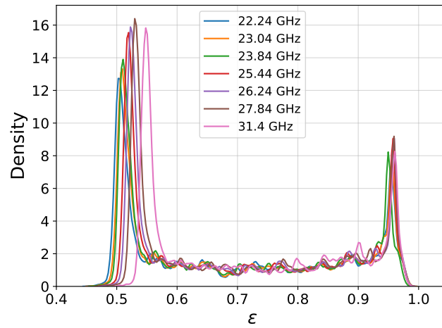
Fig. 14. Kernel density estimate of the distribution of emissivities ( \epsilon ) calculated for the frequencies between 22 and 31 GHz at a 53^\circ zenith angle for manually selected times with clear sky (N=3730).
