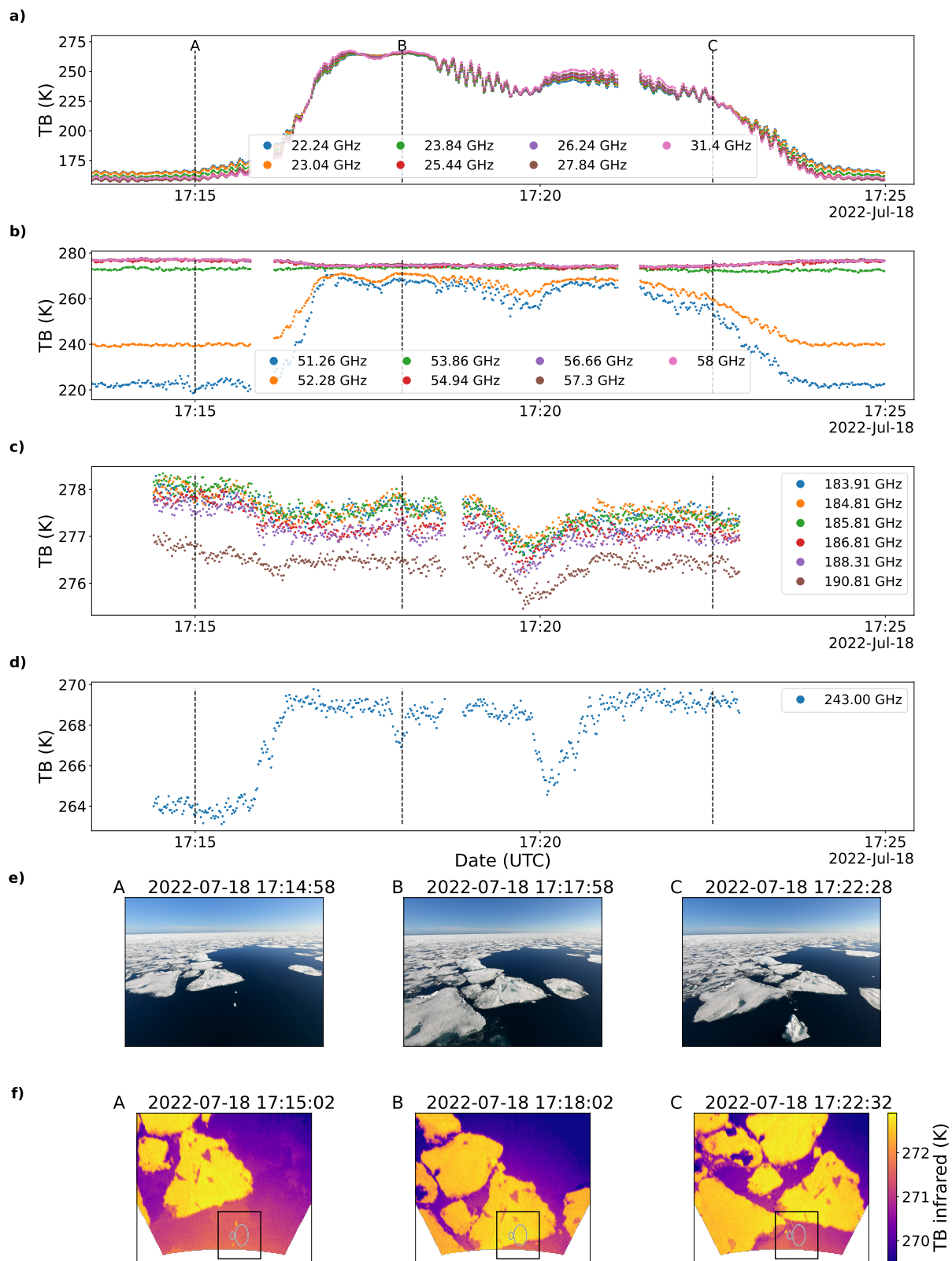
Fig. 5. HATPRO and MiRAC-P TBs on 18 July 2022 from 17:13 to 17:25 UTC for a) 22.24 to 31.4 GHz (predominantly-vertical polarization), b) 51.26 to 58 GHz (predominantly-horizontal polarization), c) 183.31 GHz (predominantly-vertical polarization) and d) 243 GHz (predominantly-horizontal polarization) measured at 53° zenith angle. The dashed vertical lines indicate the times of the e) visual and f) infrared camera images A, B, and C. The calculated footprints of the radiometers are indicated by the green ellipses in the IR imagery within the black
