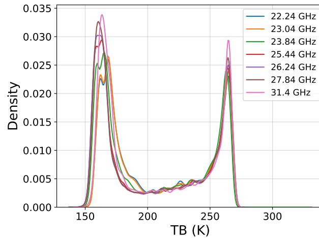
Fig. 7. All surface TB observations during ATWAICE at frequencies between 22 to 31 GHz at a 53^\circ zenith angle and predominantly-vertical polarization. The total number of measurements is 500,982 (equivalent to about 139 hours). The data is shown as probability density using kernel density estimation with a Gaussian kernel.
