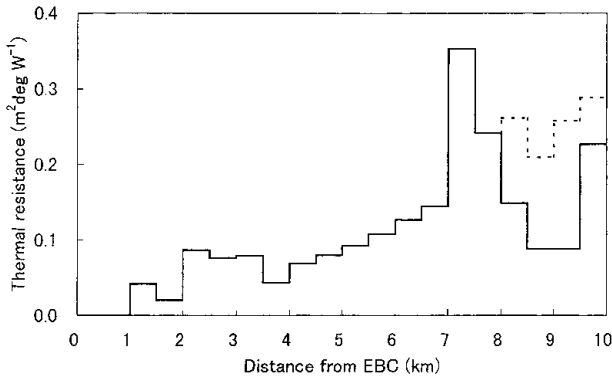
Fig. 3. Thermal resistance for every 0.5 km interval. Solid line shows calculation neglecting latent-heat flux. Dotted line that when latent-heat flux in wet areas is accounted for.
