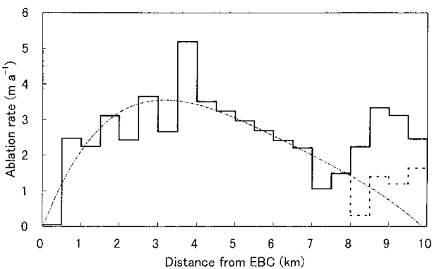
Fig. 4. Annual ablation estimated for every 0.5 km interval. Solid line shows calculation neglecting latent-heat flux. Dotted line that when latent-heat flux in wet areas is accounted for. The approximation of the profile is shown with the dash-and-dot line which is used for further calculation.
