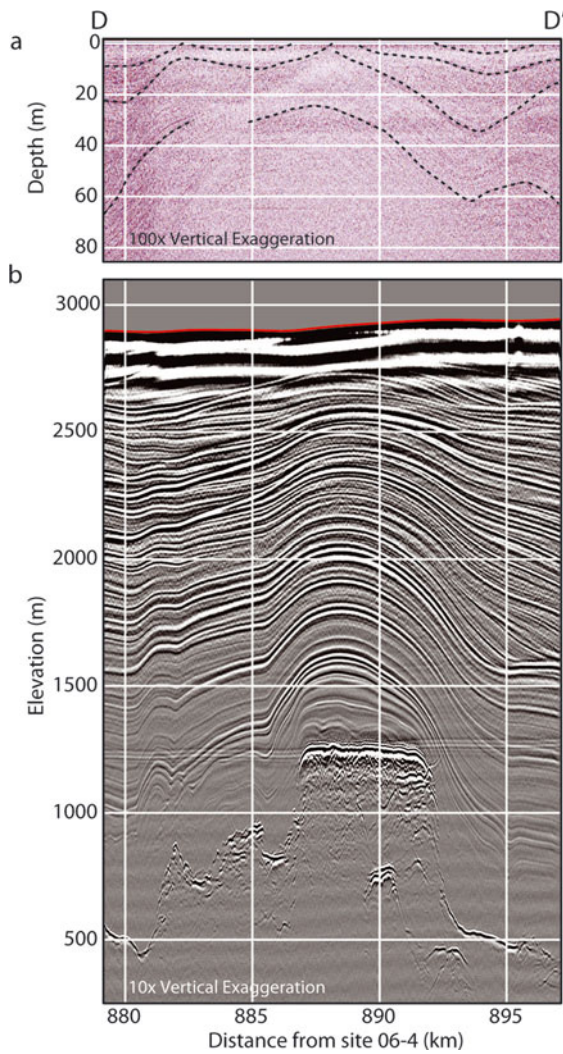
Fig. 5. Profile D–D' is an example of layers intersecting the ice surface. (a) 200 MHz data show the intersection of near-surface layers with the surface. Some prominent reflectors are highlighted. (b) Migrated and elevation-corrected 3 MHz data show that a subglacial mountain has created a vertical strain in the ice and a topographic high where aeolian erosion rates are higher. The horizontal stripes at 1200 m are an artifact of the horizontal filter.
