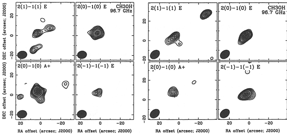
Figure 1. BIMA interferometric maps of integrated \text{CH}_3\text{OH} emission of Comet Hale-Bopp in two epochs: March 31 (left) and March 27, 1997 (right). Note the extended structure and gas clump visible at the 2_1-1_1 E1 transition to the northwest of the nucleus (marked by “+”) along the dust tail. This suggests methanol may evaporate from dust grains in the dust tail directly as predicted by grain chemistry.
