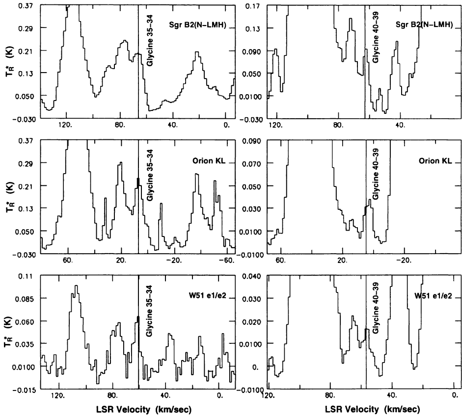
Figure 2. Sample glycine spectra at 1.4 mm (left panels) and at 1.2 mm (right panels) observed with the former NRAO 12-m telescope. Vertical lines denote the spectral lines of glycine.
