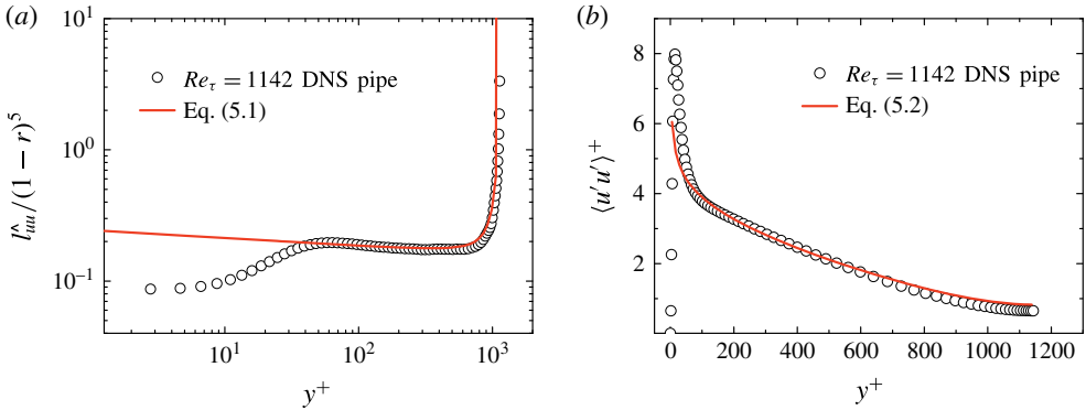
FIGURE 10. (Colour online) (a) Compensated plot of l_{uu} (divided by 1 - r^5 ) in pipe flow at Re_\tau = 1142 . DNS data (symbols) compared with (5.1) (line). (b) Outer profile of DNS \langle u'u' \rangle^+ (symbols) compared with (5.2) (line).
